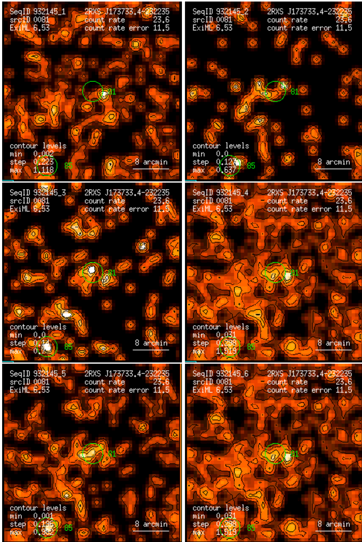
Figure 81: RASS 932145: detection 0081: band rate images, Gaussian filter: (1) PSPC channels 11 – 41, (2) 52 – 90, (3) 91 – 201, (4) 11 – 235, (5) 52 – 201, (6) 11 – 201. Broad band rates in counts/ks. Band rate contour levels in counts/ks/arcmin 2 .
