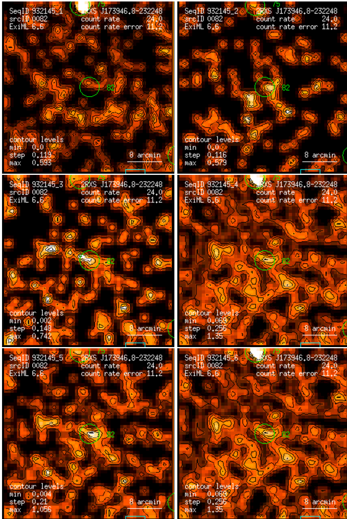
Figure 82: RASS 932145: detection 0082: band rate images, Gaussian filter: (1) PSPC channels 11 – 41, (2) 52 – 90, (3) 91 – 201, (4) 11 – 235, (5) 52 – 201, (6) 11 – 201. Broad band rates in counts/ks. Band rate contour levels in counts/ks/arcmin 2 .
