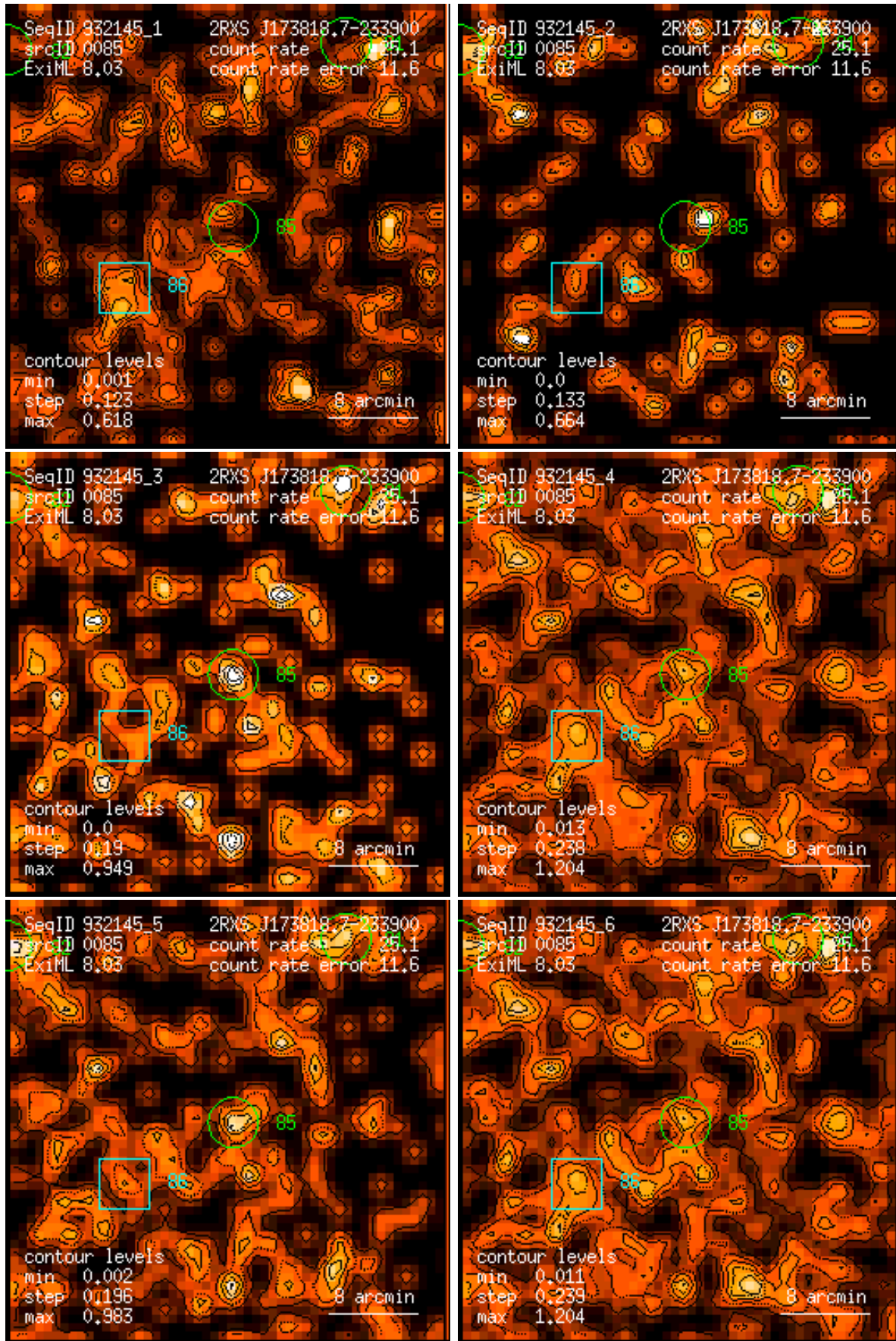
Figure 85: RASS 932145: detection 0085: band rate images, Gaussian filter: (1) PSPC channels 11 – 41, (2) 52 – 90, (3) 91 – 201, (4) 11 – 235, (5) 52 – 201, (6) 11 – 201. Broad band rates in counts/ks. Band rate contour levels in counts/ks/arcmin 2 .
