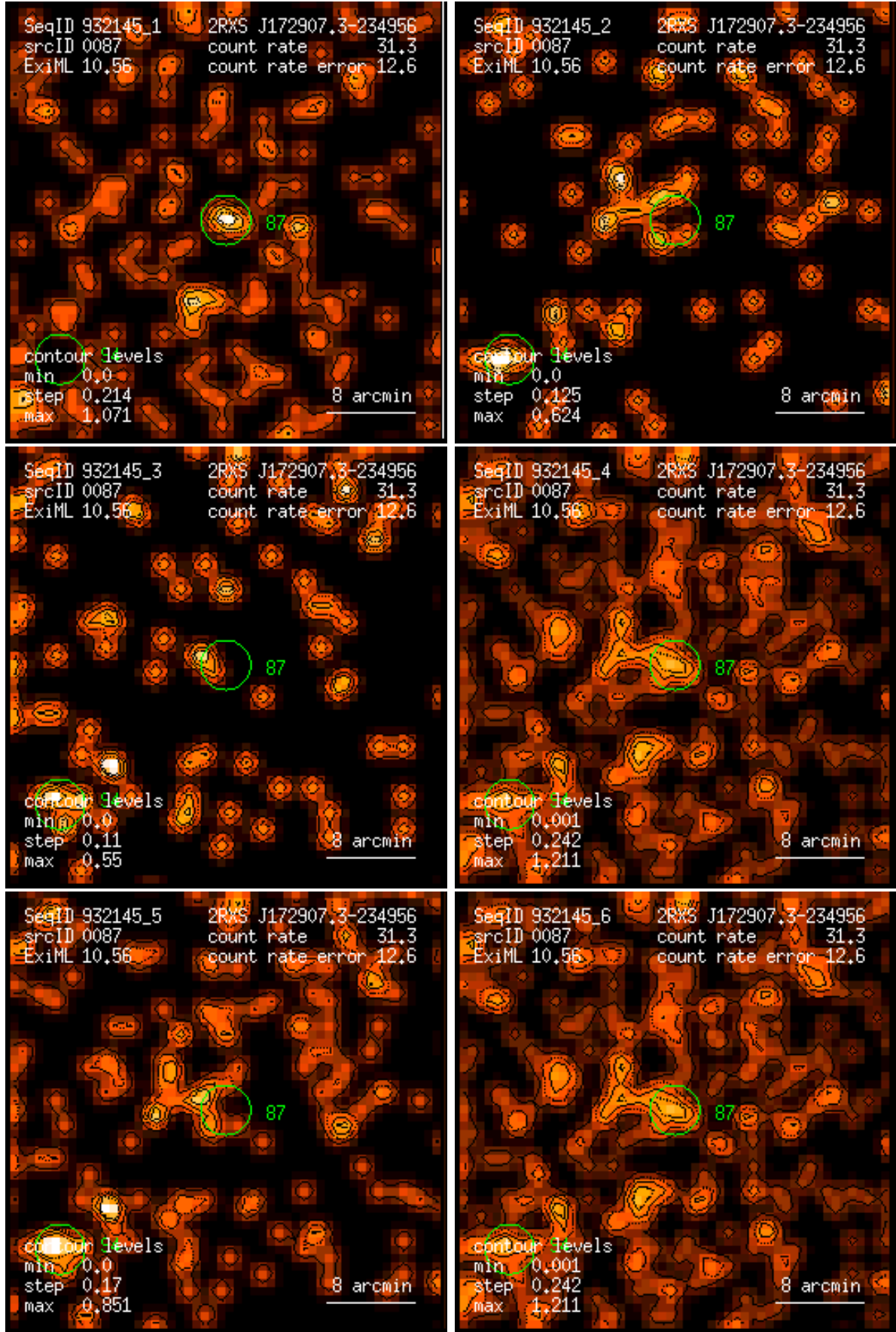
Figure 87: RASS 932145: detection 0087: band rate images, Gaussian filter: (1) PSPC channels 11 – 41, (2) 52 – 90, (3) 91 – 201, (4) 11 – 235, (5) 52 – 201, (6) 11 – 201. Broad band rates in counts/ks. Band rate contour levels in counts/ks/arcmin 2 .
