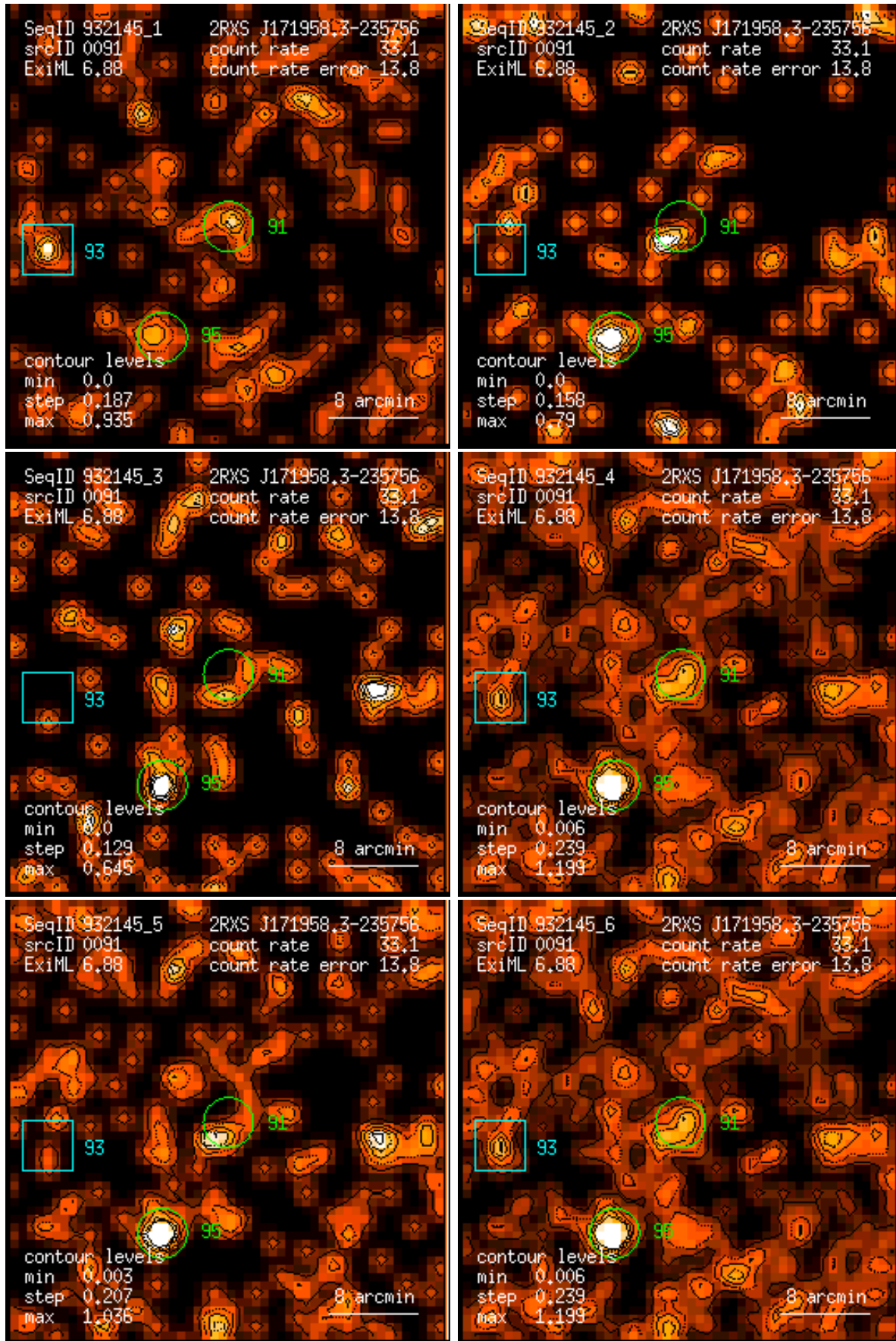
Figure 91: RASS 932145: detection 0091: band rate images, Gaussian filter: (1) PSPC channels 11 – 41, (2) 52 – 90, (3) 91 – 201, (4) 11 – 235, (5) 52 – 201, (6) 11 – 201. Broad band rates in counts/ks. Band rate contour levels in counts/ks/arcmin 2 .
