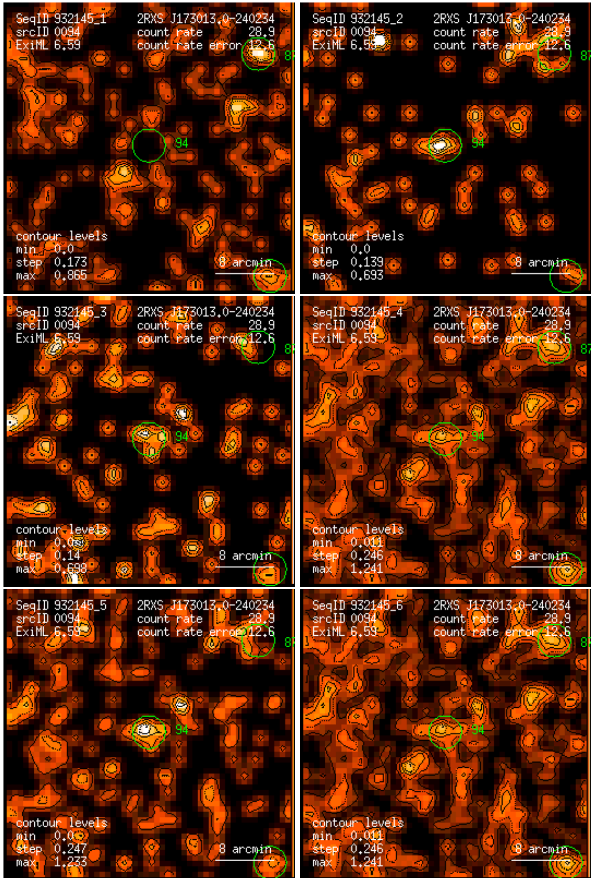
Figure 94: RASS 932145: detection 0094: band rate images, Gaussian filter: (1) PSPC channels 11 – 41, (2) 52 – 90, (3) 91 – 201, (4) 11 – 235, (5) 52 – 201, (6) 11 – 201. Broad band rates in counts/ks. Band rate contour levels in counts/ks/arcmin 2 .
