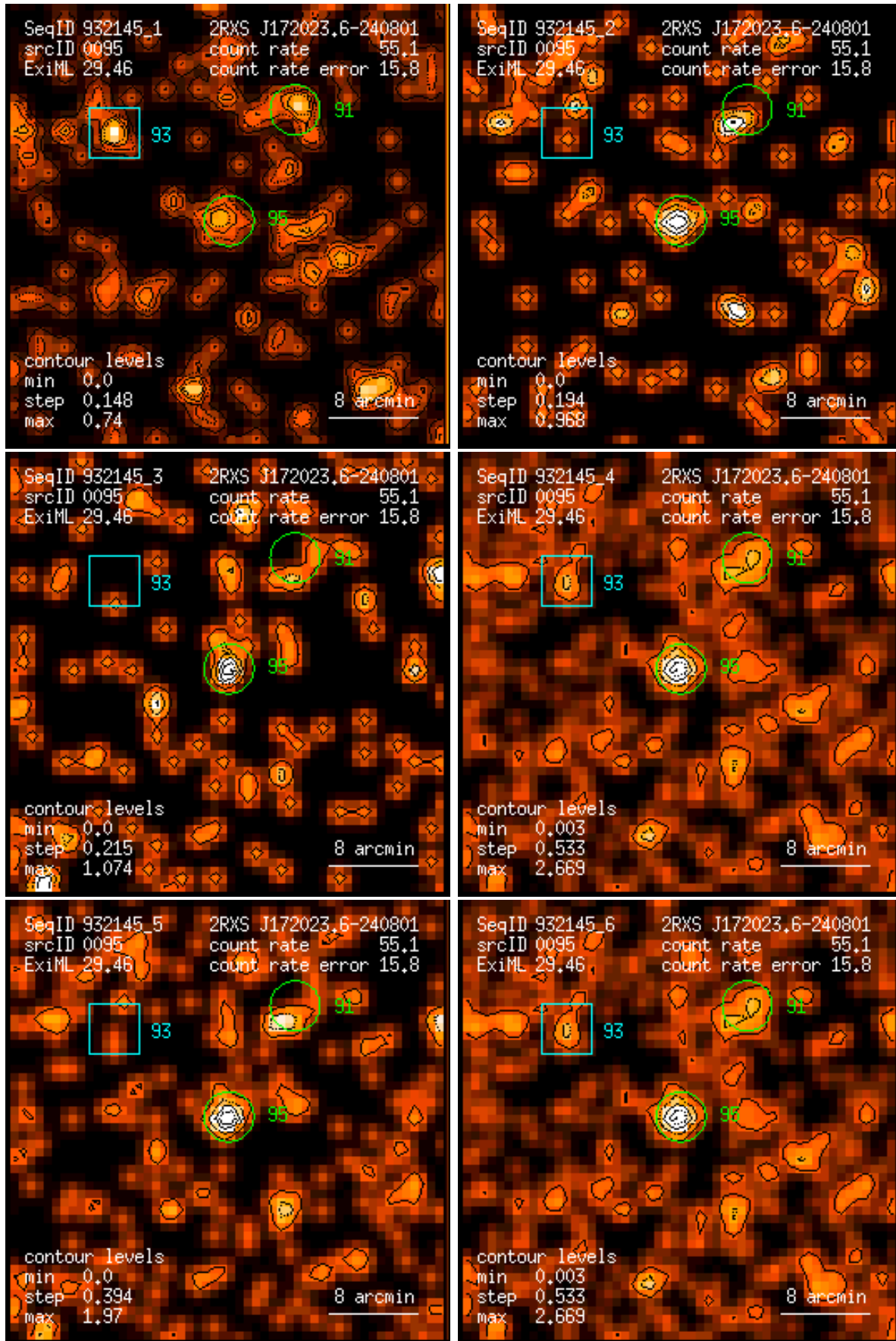
Figure 95: RASS 932145: detection 0095: band rate images, Gaussian filter: (1) PSPC channels 11 – 41, (2) 52 – 90, (3) 91 – 201, (4) 11 – 235, (5) 52 – 201, (6) 11 – 201. Broad band rates in counts/ks. Band rate contour levels in counts/ks/arcmin 2 .
