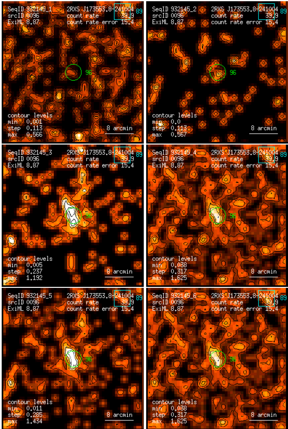
Figure 96: RASS 932145: detection 0096: band rate images, Gaussian filter: (1) PSPC channels 11 – 41, (2) 52 – 90, (3) 91 – 201, (4) 11 – 235, (5) 52 – 201, (6) 11 – 201. Broad band rates in counts/ks. Band rate contour levels in counts/ks/arcmin 2 .
