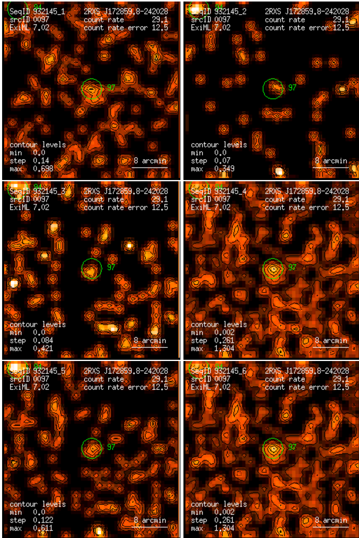
Figure 97: RASS 932145: detection 0097: band rate images, Gaussian filter: (1) PSPC channels 11 – 41, (2) 52 – 90, (3) 91 – 201, (4) 11 – 235, (5) 52 – 201, (6) 11 – 201. Broad band rates in counts/ks. Band rate contour levels in counts/ks/arcmin 2 .
