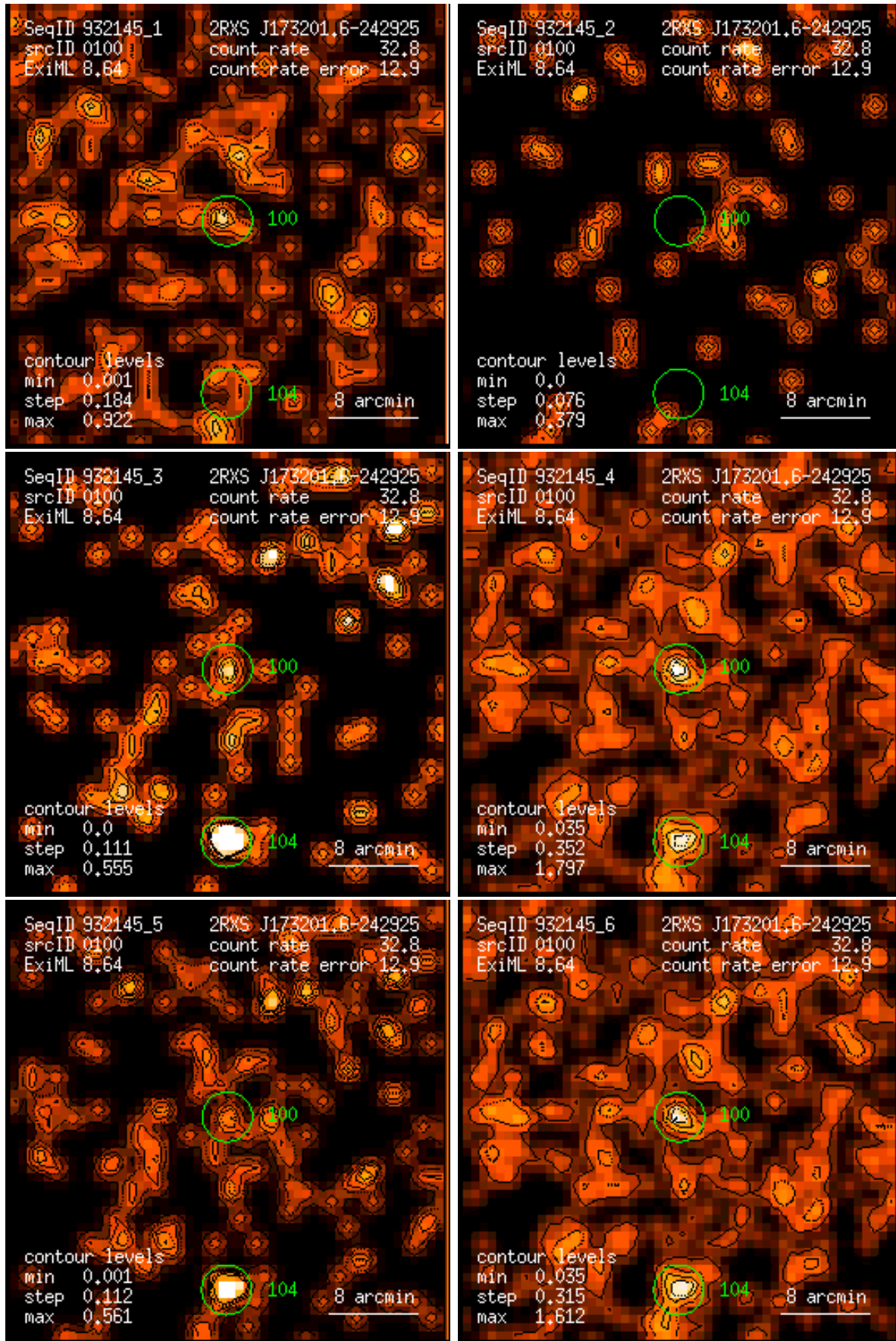
Figure 100: RASS 932145: detection 0100: band rate images, Gaussian filter: (1) PSPC channels 11 – 41, (2) 52 – 90, (3) 91 – 201, (4) 11 – 235, (5) 52 – 201, (6) 11 – 201. Broad band rates in counts/ks. Band rate contour levels in counts/ks/arcmin 2 .
