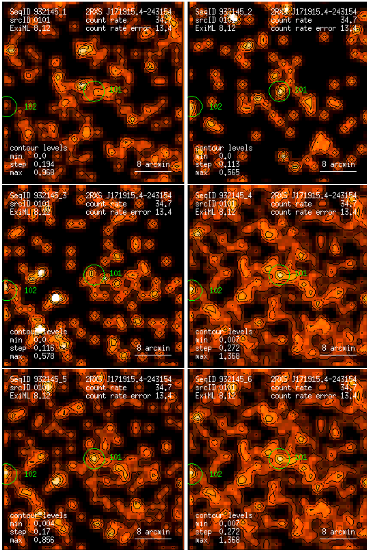
Figure 101: RASS 932145: detection 0101: band rate images, Gaussian filter: (1) PSPC channels 11 – 41, (2) 52 – 90, (3) 91 – 201, (4) 11 – 235, (5) 52 – 201, (6) 11 – 201. Broad band rates in counts/ks. Band rate contour levels in counts/ks/arcmin 2 .
