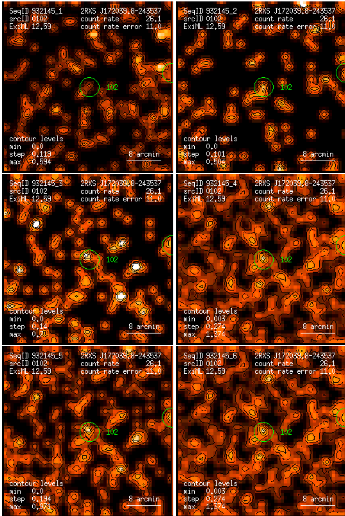
Figure 102: RASS 932145: detection 0102: band rate images, Gaussian filter: (1) PSPC channels 11 – 41, (2) 52 – 90, (3) 91 – 201, (4) 11 – 235, (5) 52 – 201, (6) 11 – 201. Broad band rates in counts/ks. Band rate contour levels in counts/ks/arcmin 2 .
