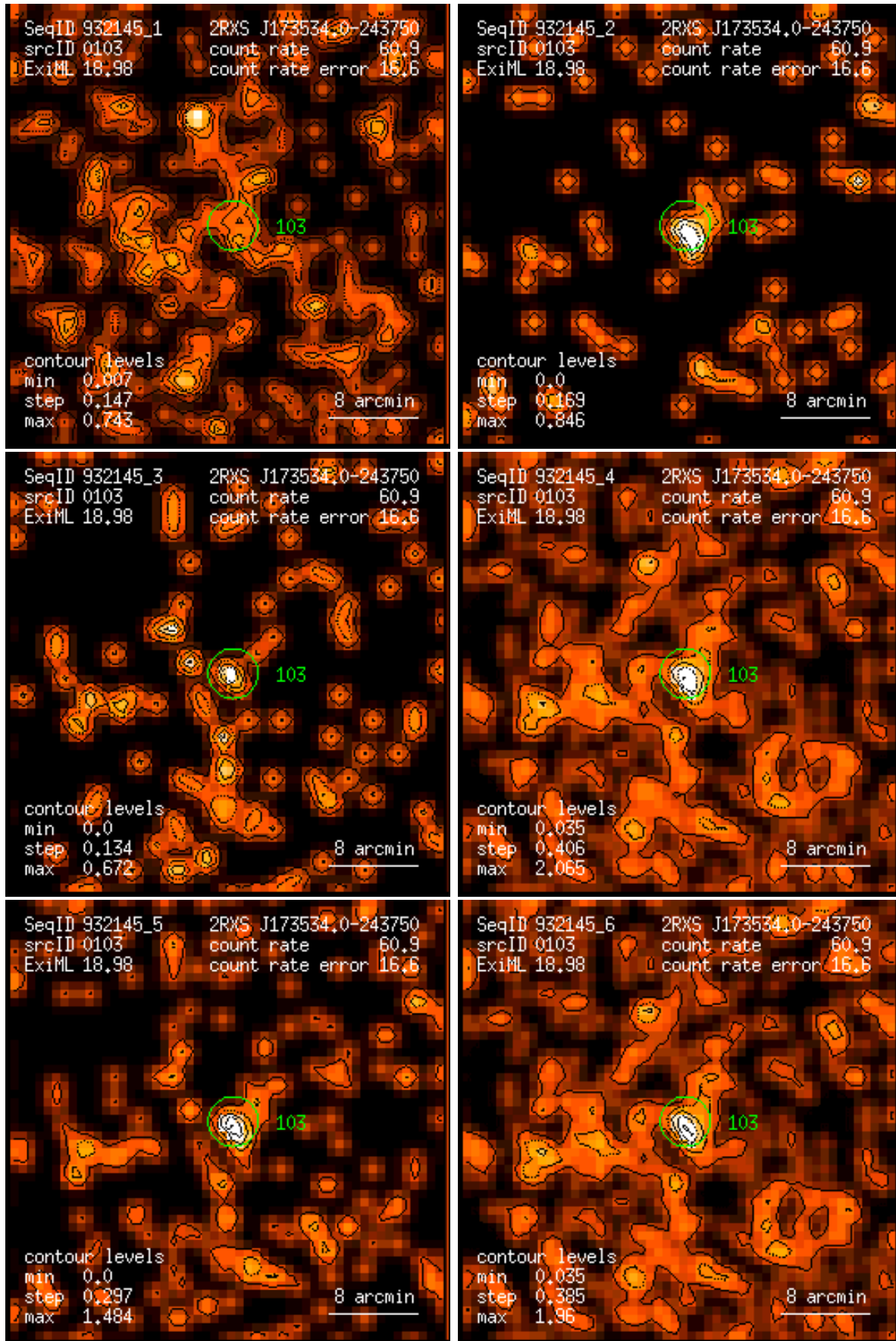
Figure 103: RASS 932145: detection 0103: band rate images, Gaussian filter: (1) PSPC channels 11 – 41, (2) 52 – 90, (3) 91 – 201, (4) 11 – 235, (5) 52 – 201, (6) 11 – 201. Broad band rates in counts/ks. Band rate contour levels in counts/ks/arcmin 2 .
