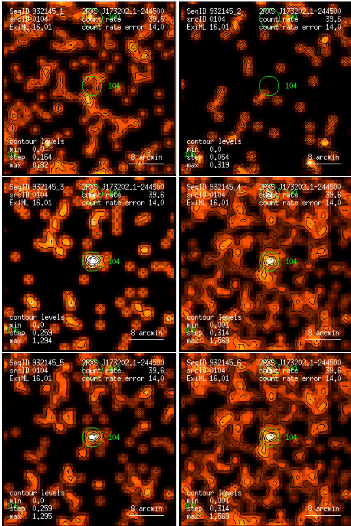
Figure 104: RASS 932145: detection 0104: band rate images, Gaussian filter: (1) PSPC channels 11 – 41, (2) 52 – 90, (3) 91 – 201, (4) 11 – 235, (5) 52 – 201, (6) 11 – 201. Broad band rates in counts/ks. Band rate contour levels in counts/ks/arcmin 2 .
