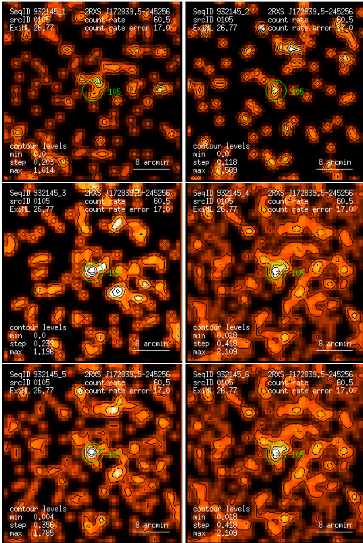
Figure 105: RASS 932145: detection 0105: band rate images, Gaussian filter: (1) PSPC channels 11 – 41, (2) 52 – 90, (3) 91 – 201, (4) 11 – 235, (5) 52 – 201, (6) 11 – 201. Broad band rates in counts/ks. Band rate contour levels in counts/ks/arcmin 2 .
