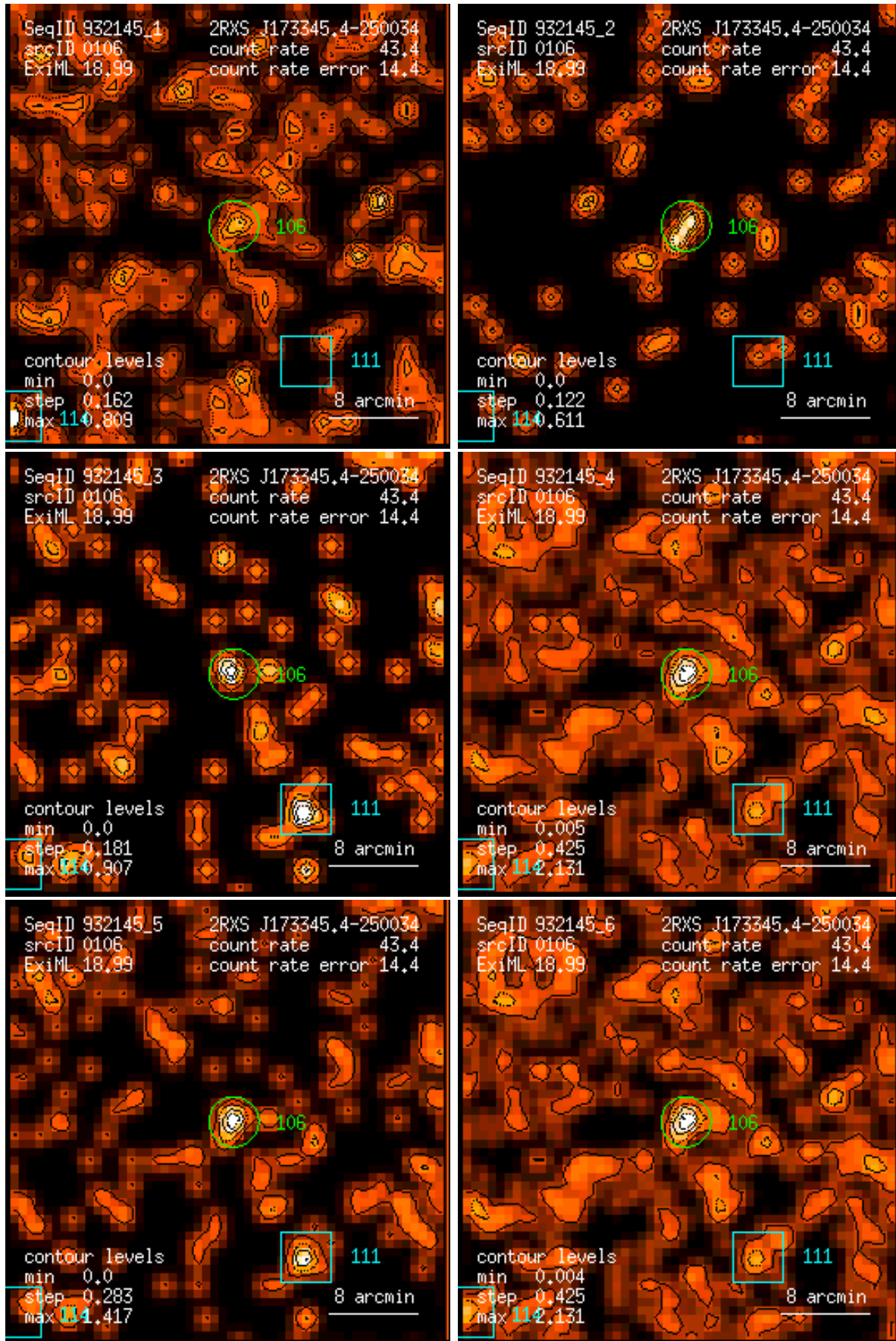
Figure 106: RASS 932145: detection 0106: band rate images, Gaussian filter: (1) PSPC channels 11 – 41, (2) 52 – 90, (3) 91 – 201, (4) 11 – 235, (5) 52 – 201, (6) 11 – 201. Broad band rates in counts/ks. Band rate contour levels in counts/ks/arcmin 2 .
