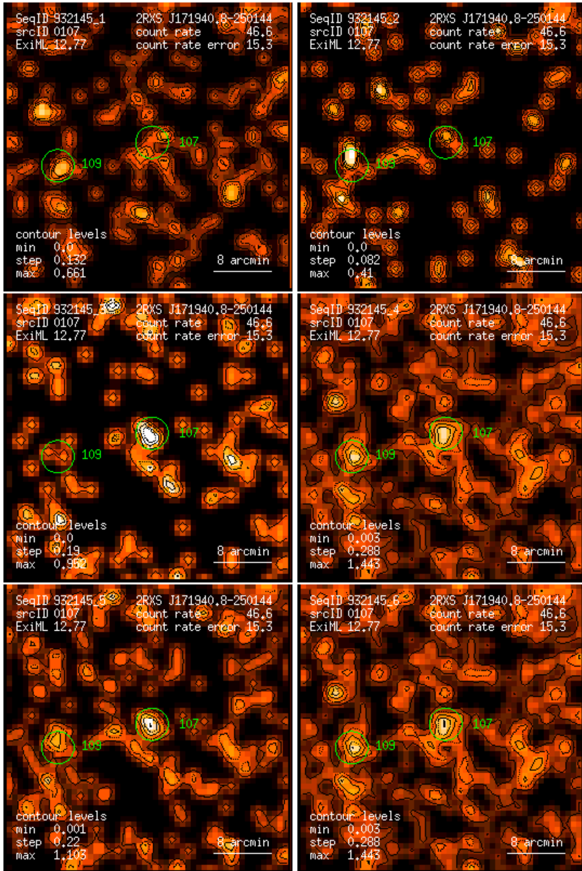
Figure 107: RASS 932145: detection 0107: band rate images, Gaussian filter: (1) PSPC channels 11 – 41, (2) 52 – 90, (3) 91 – 201, (4) 11 – 235, (5) 52 – 201, (6) 11 – 201. Broad band rates in counts/ks. Band rate contour levels in counts/ks/arcmin 2 .
