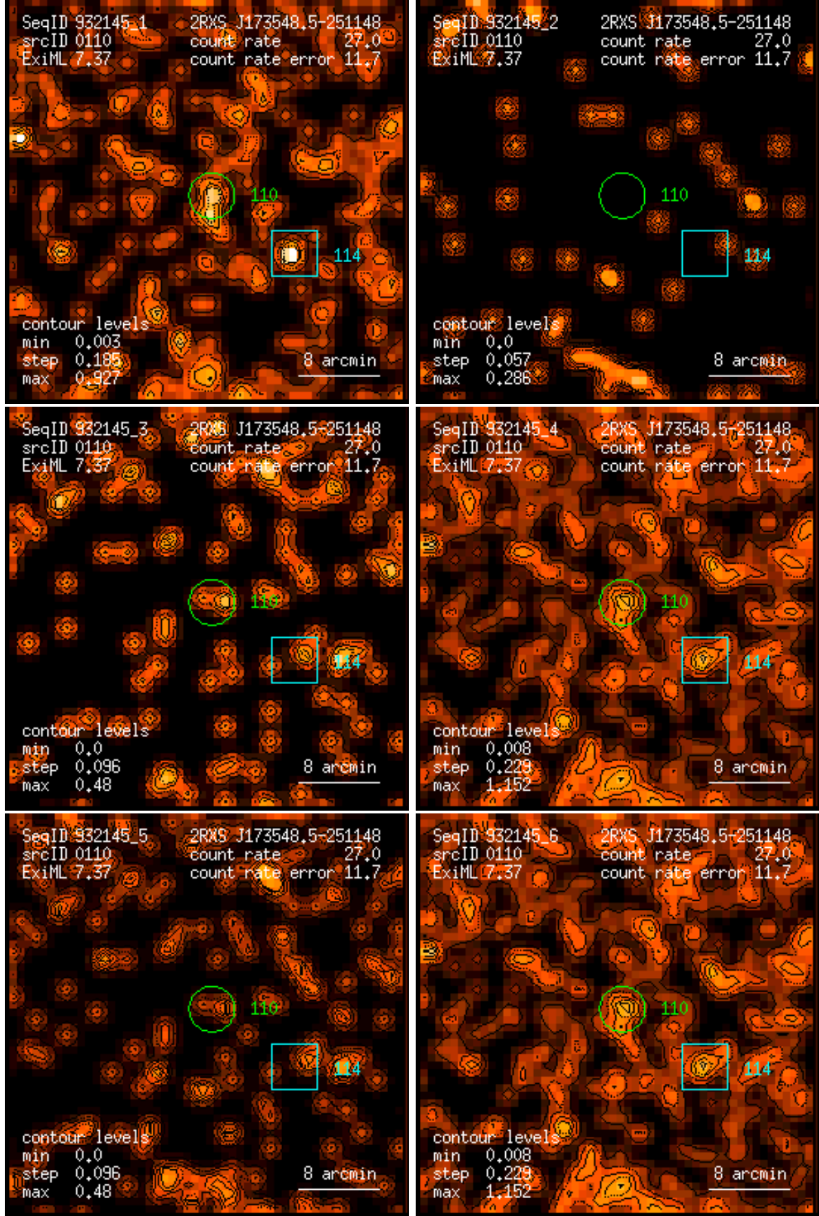
Figure 110: RASS 932145: detection 0110: band rate images, Gaussian filter: (1) PSPC channels 11 – 41, (2) 52 – 90, (3) 91 – 201, (4) 11 – 235, (5) 52 – 201, (6) 11 – 201. Broad band rates in counts/ks. Band rate contour levels in counts/ks/arcmin 2 .
