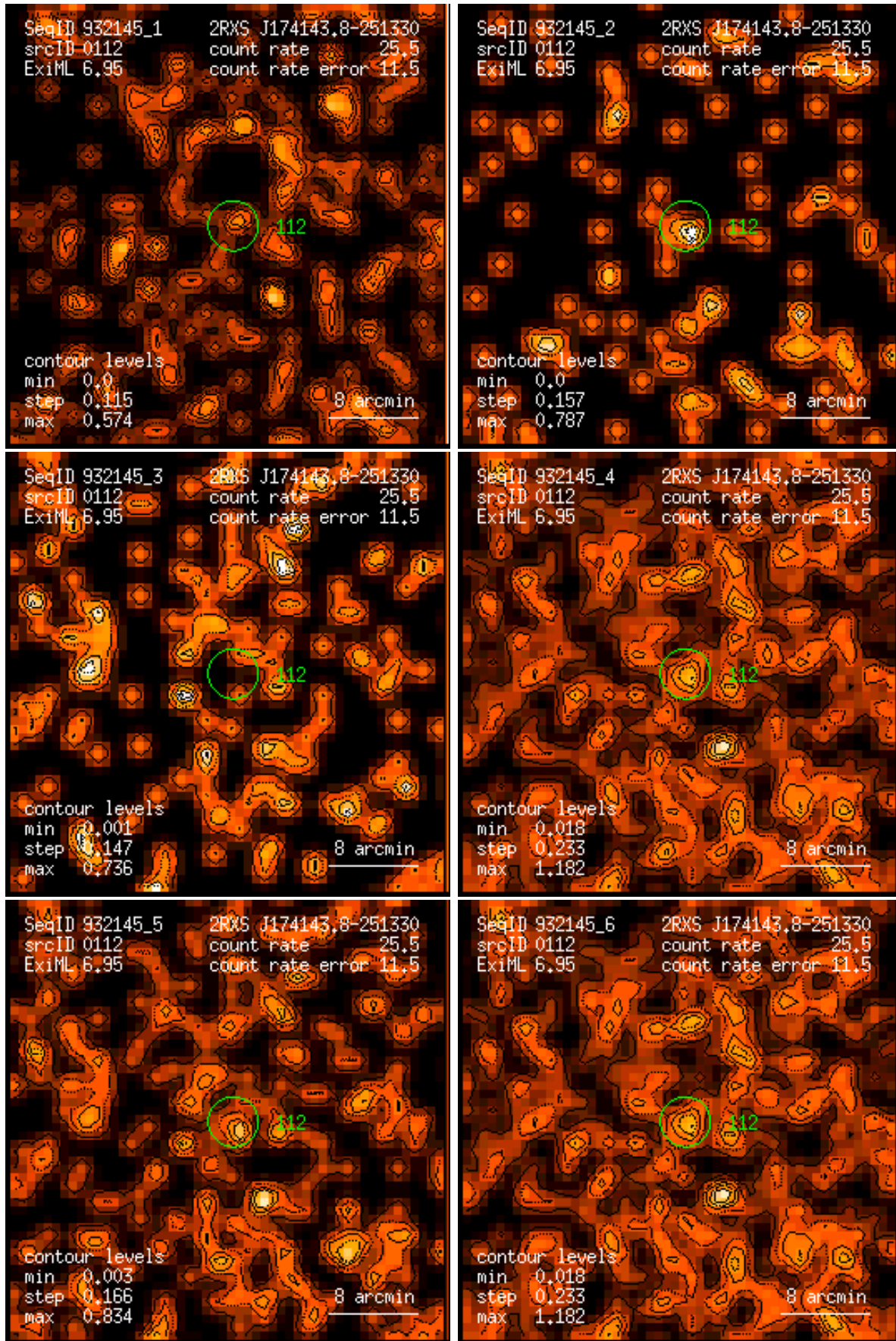
Figure 112: RASS 932145: detection 0112: band rate images, Gaussian filter: (1) PSPC channels 11 – 41, (2) 52 – 90, (3) 91 – 201, (4) 11 – 235, (5) 52 – 201, (6) 11 – 201. Broad band rates in counts/ks. Band rate contour levels in counts/ks/arcmin 2 .
