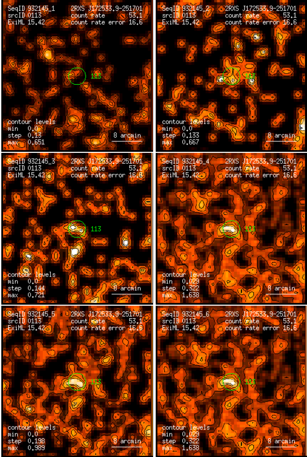
Figure 113: RASS 932145: detection 0113: band rate images, Gaussian filter: (1) PSPC channels 11 – 41, (2) 52 – 90, (3) 91 – 201, (4) 11 – 235, (5) 52 – 201, (6) 11 – 201. Broad band rates in counts/ks. Band rate contour levels in counts/ks/arcmin 2 .
