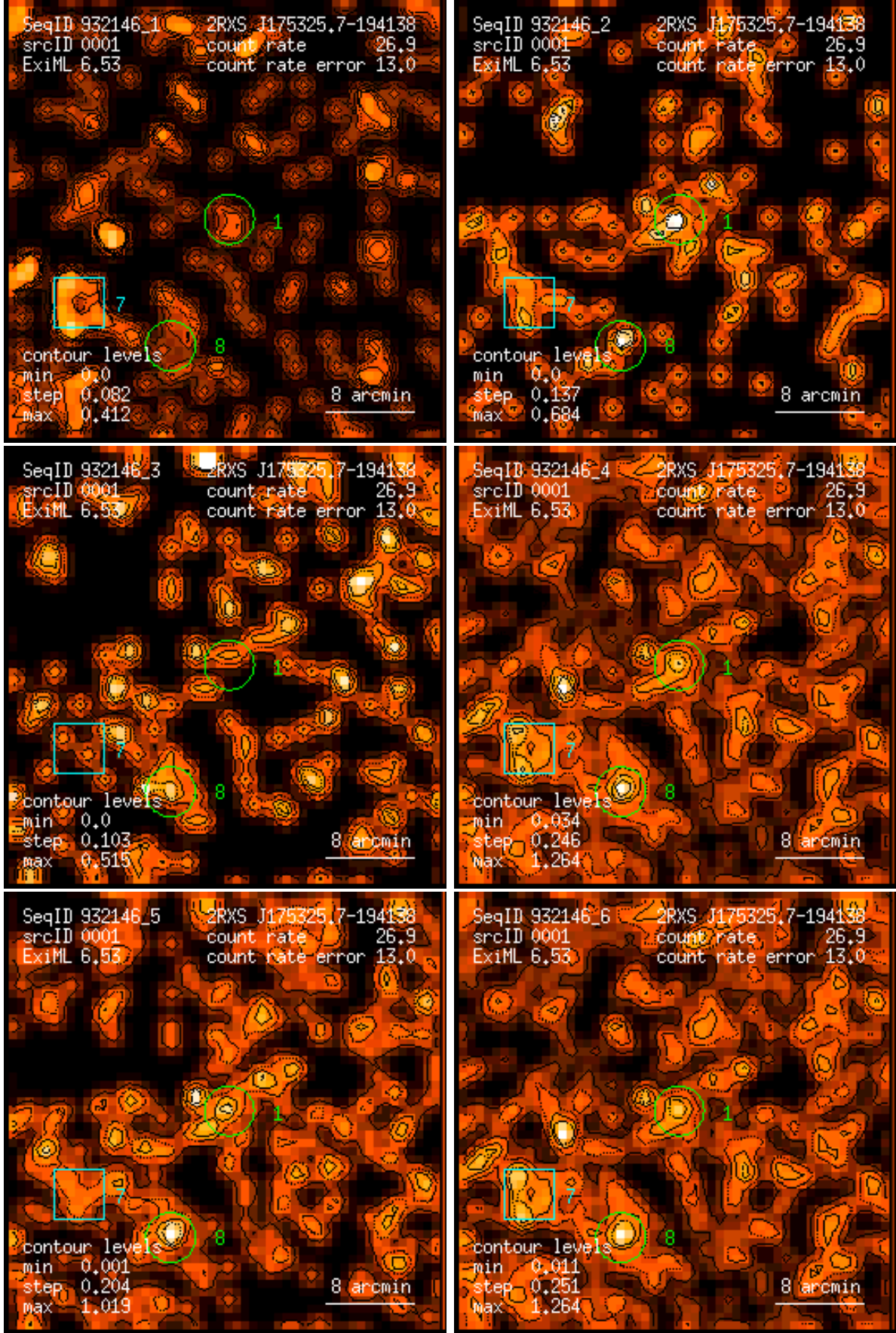
Figure 1: RASS 932146: detection 0001: band rate images, Gaussian filter: (1) PSPC channels 11 – 41, (2) 52 – 90, (3) 91 – 201, (4) 11 – 235, (5) 52 – 201, (6) 11 – 201. Broad band rates in counts/ks. Band rate contour levels in counts/ks/arcmin 2 .
