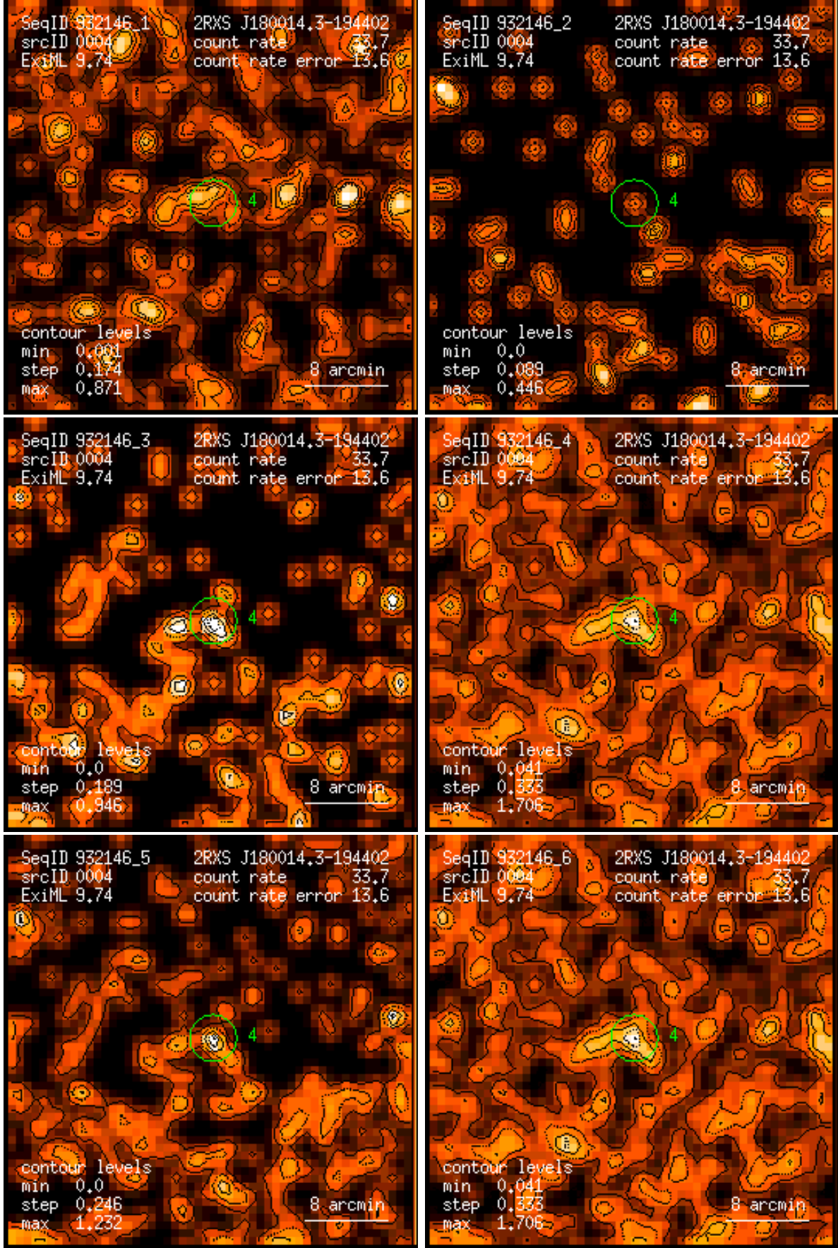
Figure 4: RASS 932146: detection 0004: band rate images, Gaussian filter: (1) PSPC channels 11 – 41, (2) 52 – 90, (3) 91 – 201, (4) 11 – 235, (5) 52 – 201, (6) 11 – 201. Broad band rates in counts/ks. Band rate contour levels in counts/ks/arcmin 2 .
