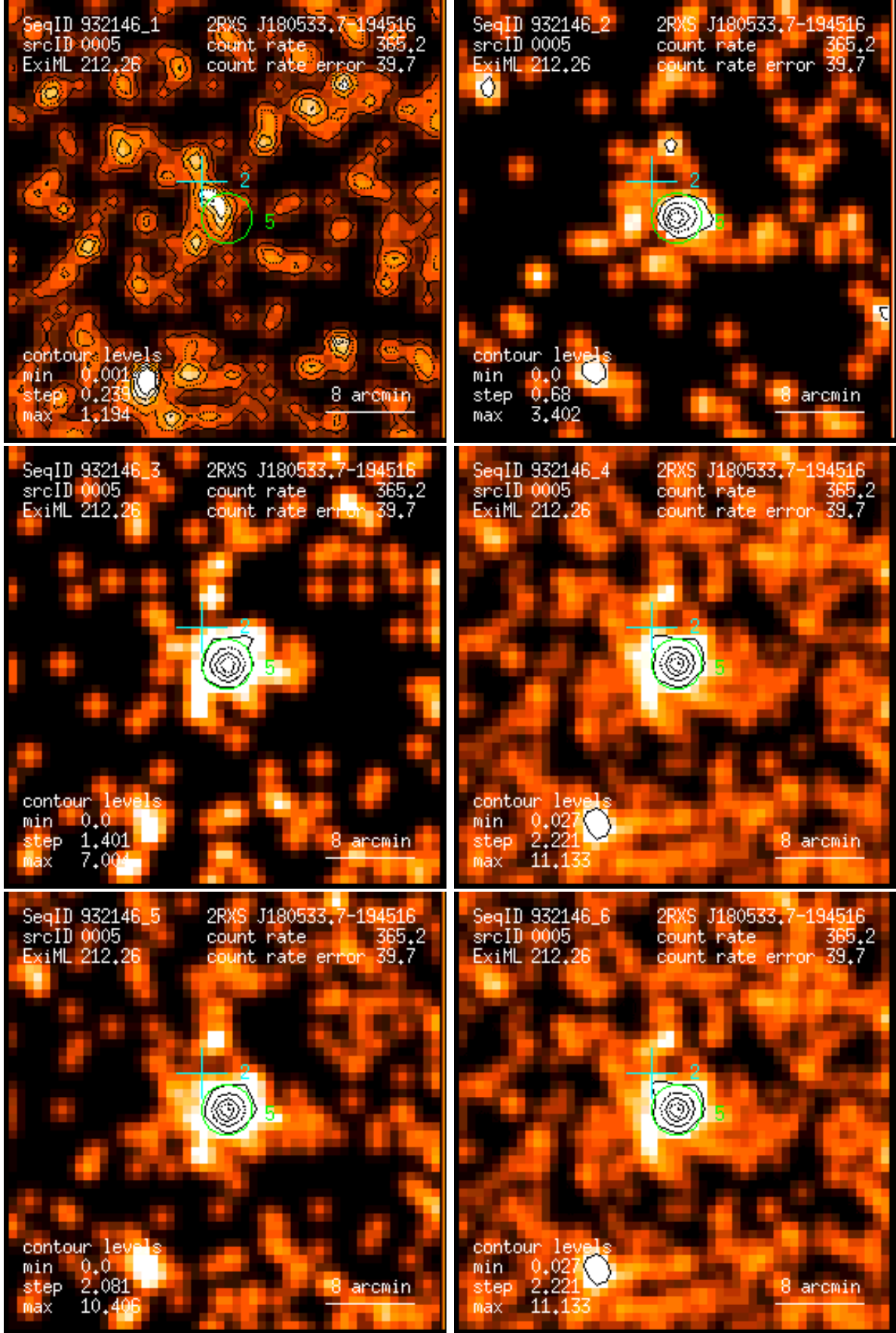
Figure 5: RASS 932146: detection 0005: band rate images, Gaussian filter: (1) PSPC channels 11 – 41, (2) 52 – 90, (3) 91 – 201, (4) 11 – 235, (5) 52 – 201, (6) 11 – 201. Broad band rates in counts/ks. Band rate contour levels in counts/ks/arcmin 2 .
