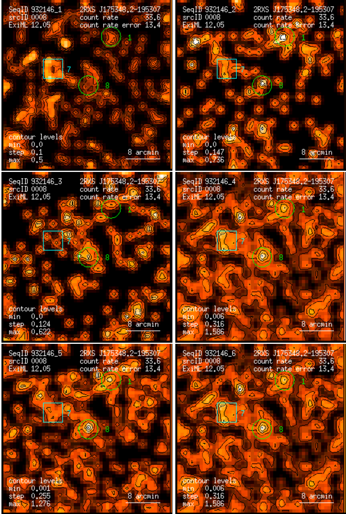
Figure 8: RASS 932146: detection 0008: band rate images, Gaussian filter: (1) PSPC channels 11 – 41, (2) 52 – 90, (3) 91 – 201, (4) 11 – 235, (5) 52 – 201, (6) 11 – 201. Broad band rates in counts/ks. Band rate contour levels in counts/ks/arcmin 2 .
