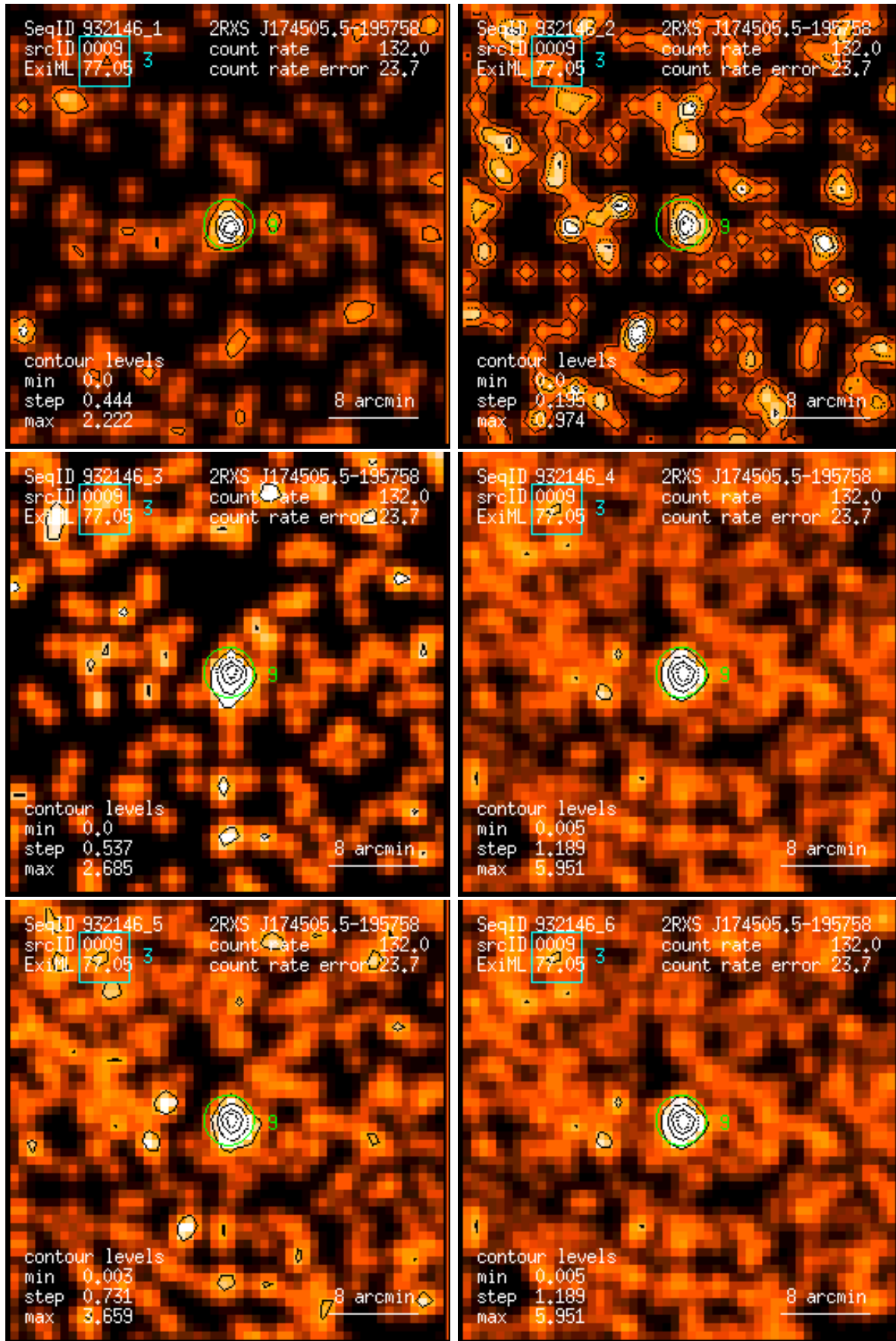
Figure 9: RASS 932146: detection 0009: band rate images, Gaussian filter: (1) PSPC channels 11 – 41, (2) 52 – 90, (3) 91 – 201, (4) 11 – 235, (5) 52 – 201, (6) 11 – 201. Broad band rates in counts/ks. Band rate contour levels in counts/ks/arcmin 2 .
