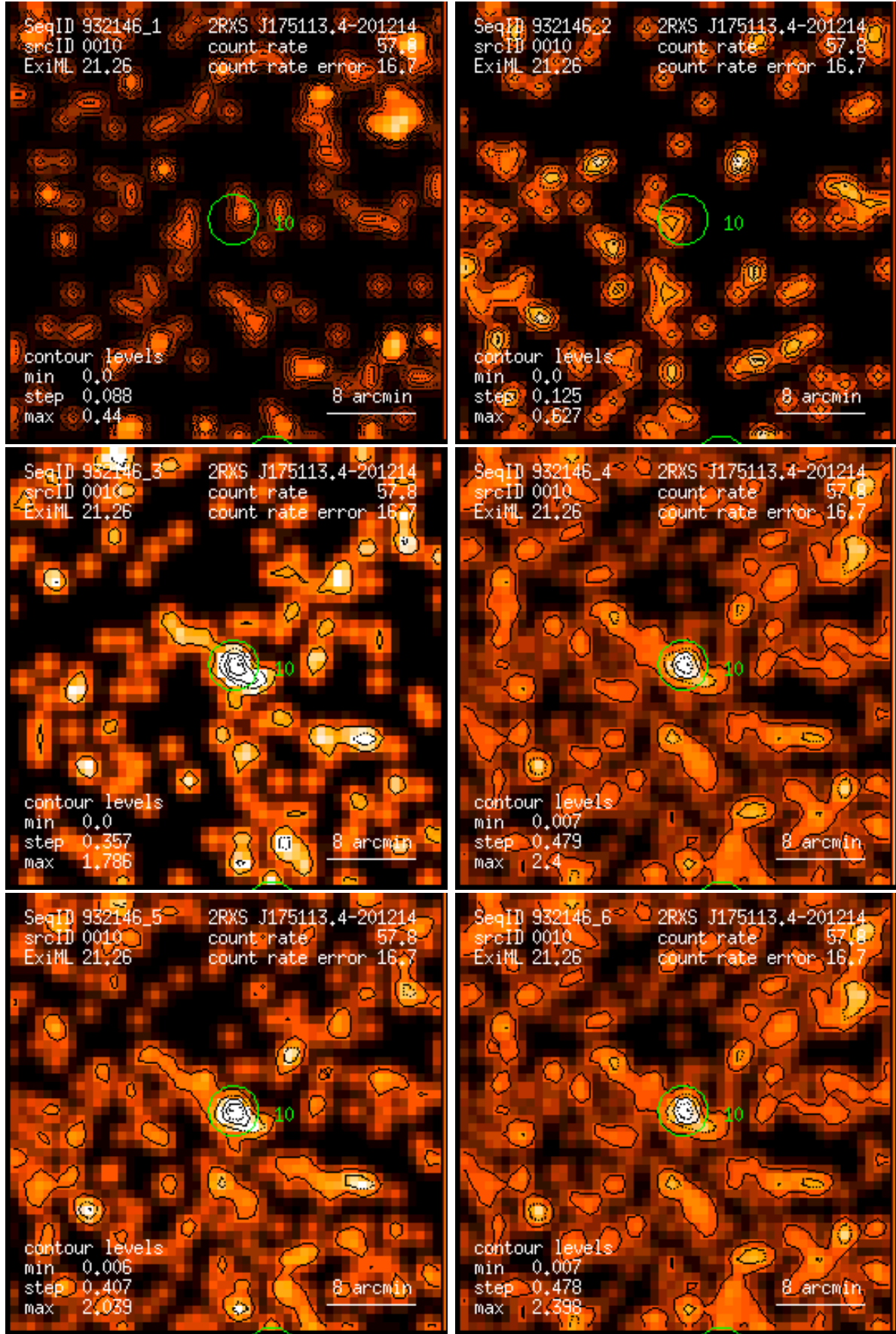
Figure 10: RASS 932146: detection 0010: band rate images, Gaussian filter: (1) PSPC channels 11 – 41, (2) 52 – 90, (3) 91 – 201, (4) 11 – 235, (5) 52 – 201, (6) 11 – 201. Broad band rates in counts/ks. Band rate contour levels in counts/ks/arcmin 2 .
