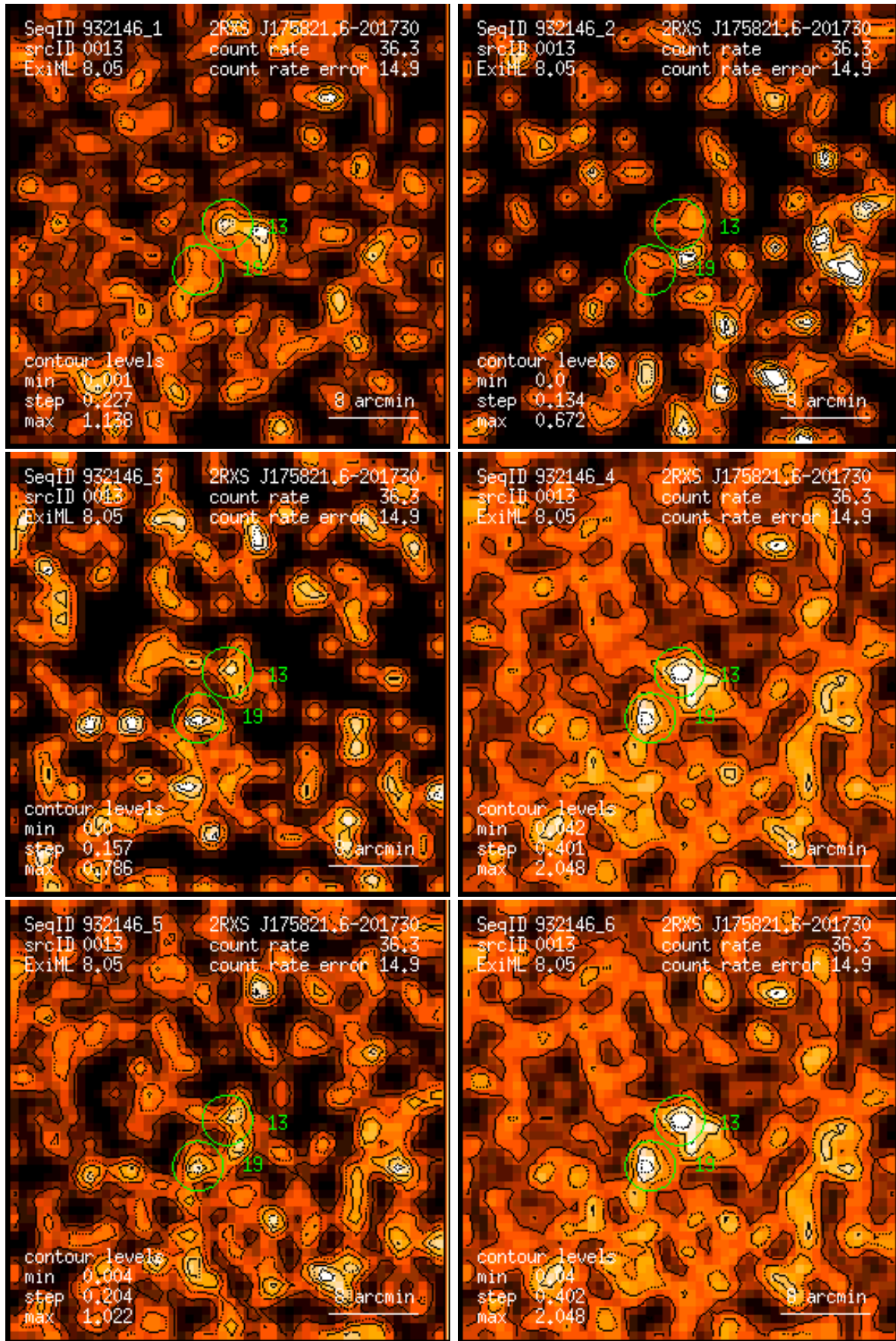
Figure 13: RASS 932146: detection 0013: band rate images, Gaussian filter: (1) PSPC channels 11 – 41, (2) 52 – 90, (3) 91 – 201, (4) 11 – 235, (5) 52 – 201, (6) 11 – 201. Broad band rates in counts/ks. Band rate contour levels in counts/ks/arcmin 2 .
