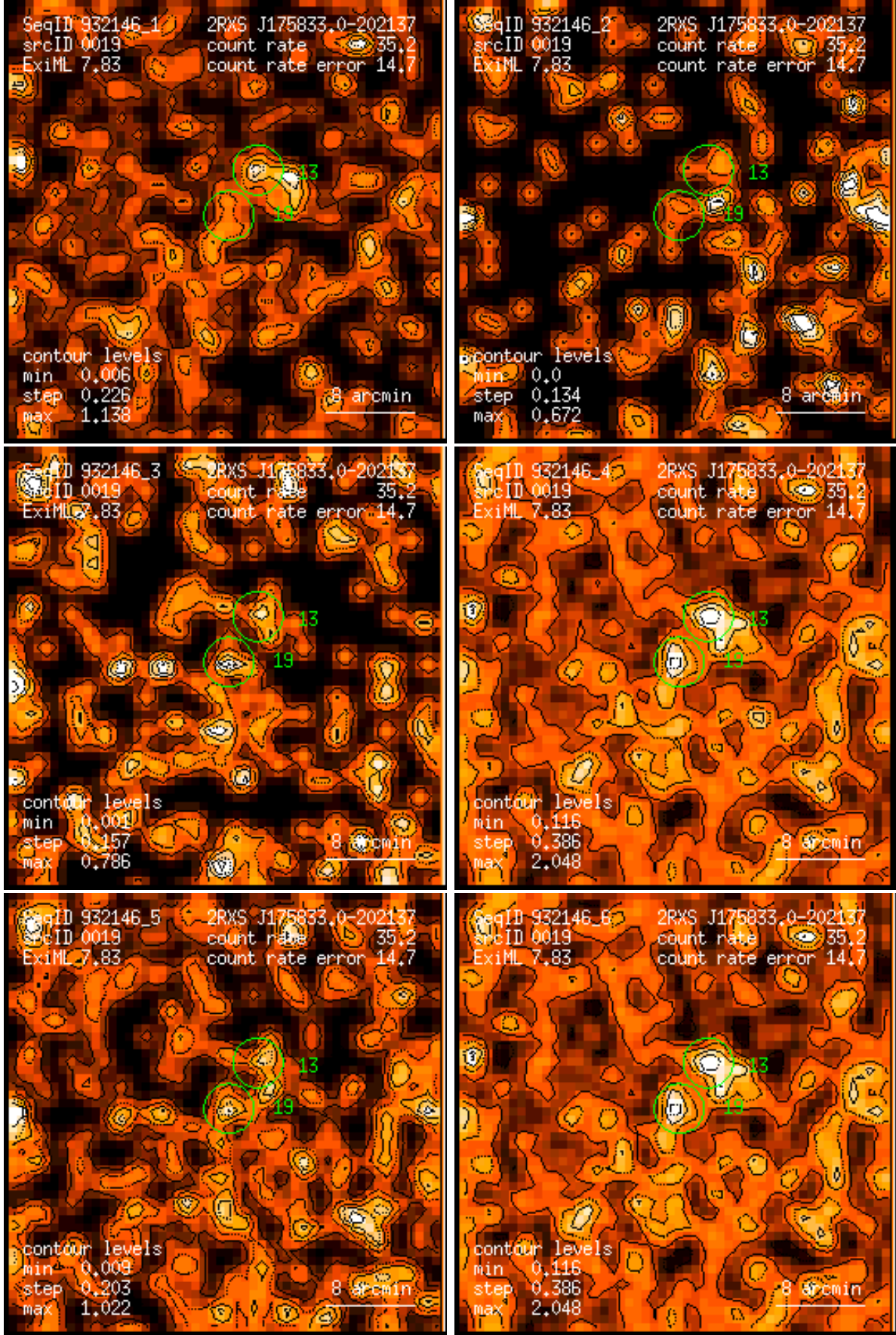
Figure 19: RASS 932146: detection 0019: band rate images, Gaussian filter: (1) PSPC channels 11 – 41, (2) 52 – 90, (3) 91 – 201, (4) 11 – 235, (5) 52 – 201, (6) 11 – 201. Broad band rates in counts/ks. Band rate contour levels in counts/ks/arcmin 2 .
