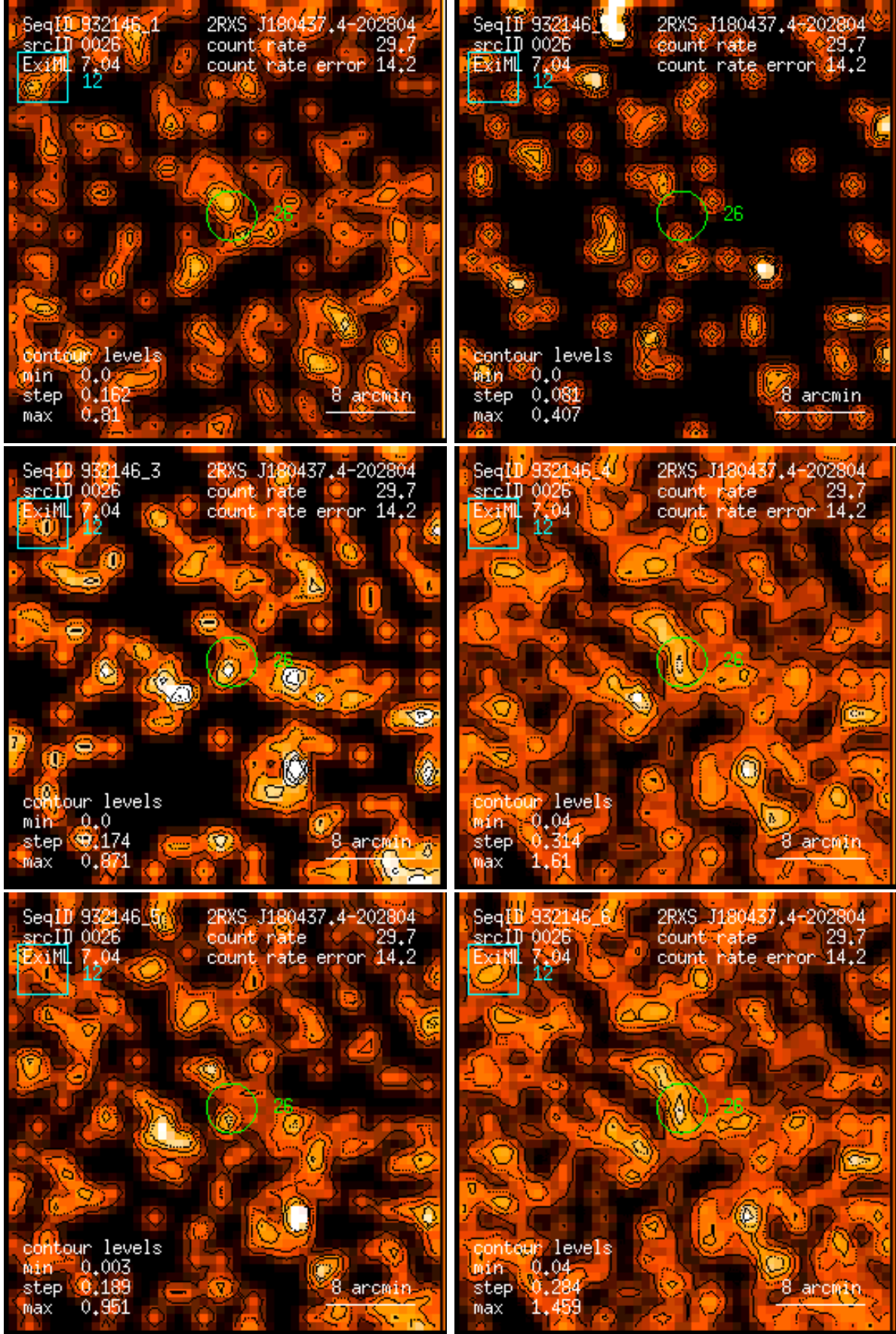
Figure 26: RASS 932146: detection 0026: band rate images, Gaussian filter: (1) PSPC channels 11 – 41, (2) 52 – 90, (3) 91 – 201, (4) 11 – 235, (5) 52 – 201, (6) 11 – 201. Broad band rates in counts/ks. Band rate contour levels in counts/ks/arcmin 2 .
