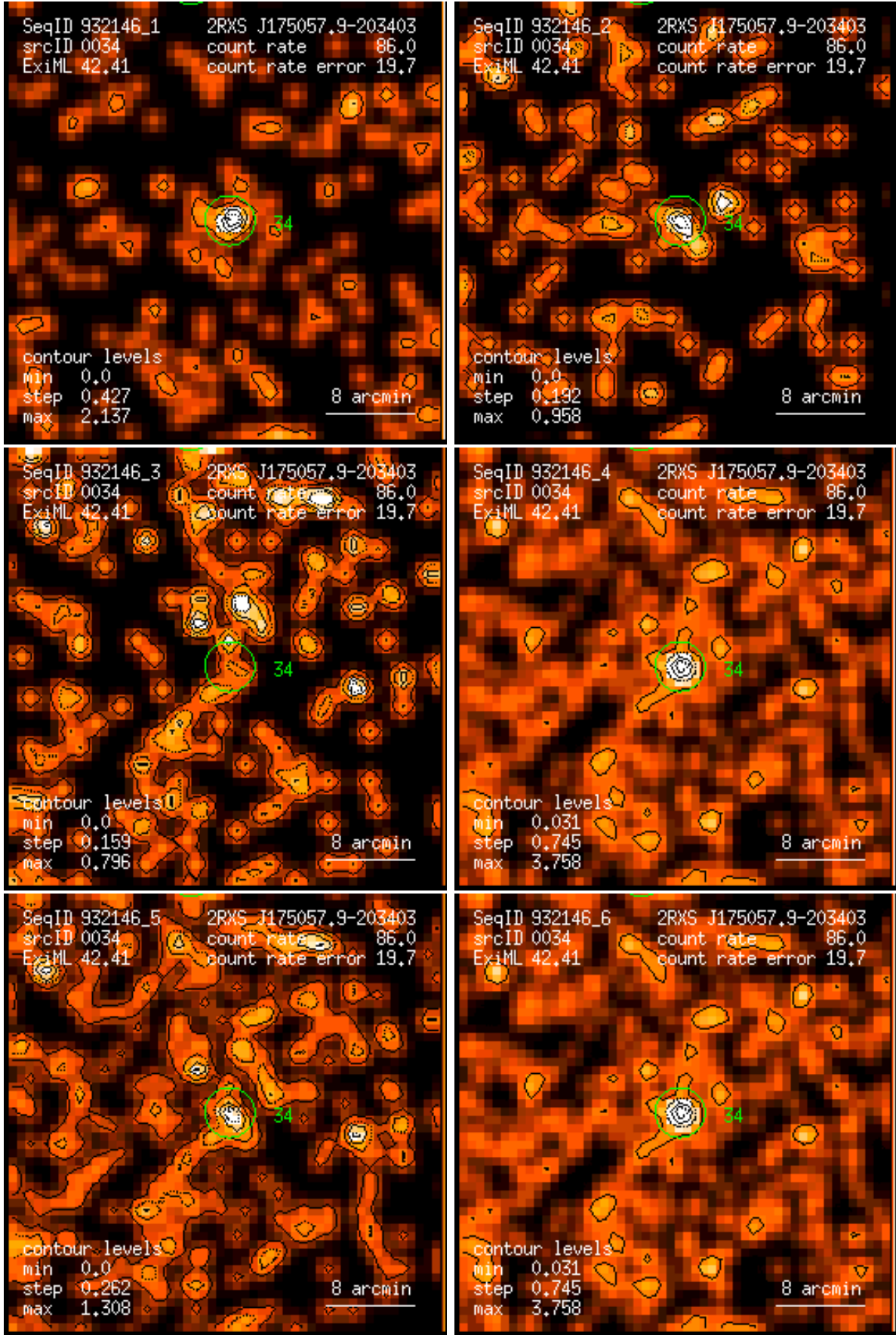
Figure 34: RASS 932146: detection 0034: band rate images, Gaussian filter: (1) PSPC channels 11 – 41, (2) 52 – 90, (3) 91 – 201, (4) 11 – 235, (5) 52 – 201, (6) 11 – 201. Broad band rates in counts/ks. Band rate contour levels in counts/ks/arcmin 2 .
