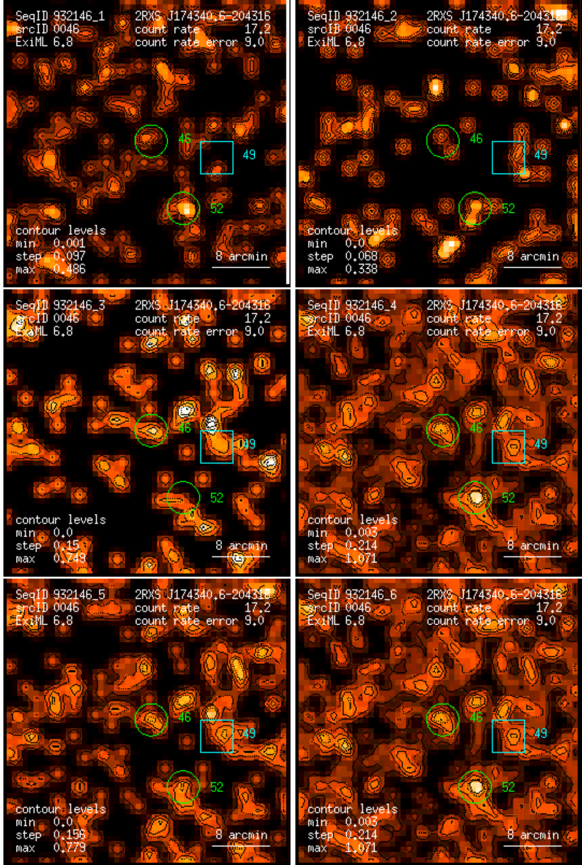
Figure 46: RASS 932146: detection 0046: band rate images, Gaussian filter: (1) PSPC channels 11 – 41, (2) 52 – 90, (3) 91 – 201, (4) 11 – 235, (5) 52 – 201, (6) 11 – 201. Broad band rates in counts/ks. Band rate contour levels in counts/ks/arcmin 2 .
