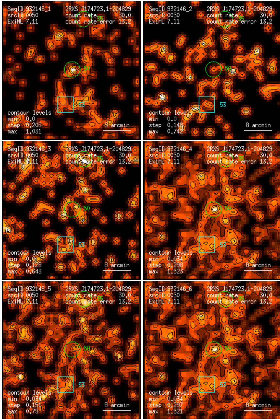
Figure 50: RASS 932146: detection 0050: band rate images, Gaussian filter: (1) PSPC channels 11 – 41, (2) 52 – 90, (3) 91 – 201, (4) 11 – 235, (5) 52 – 201, (6) 11 – 201. Broad band rates in counts/ks. Band rate contour levels in counts/ks/arcmin 2 .
