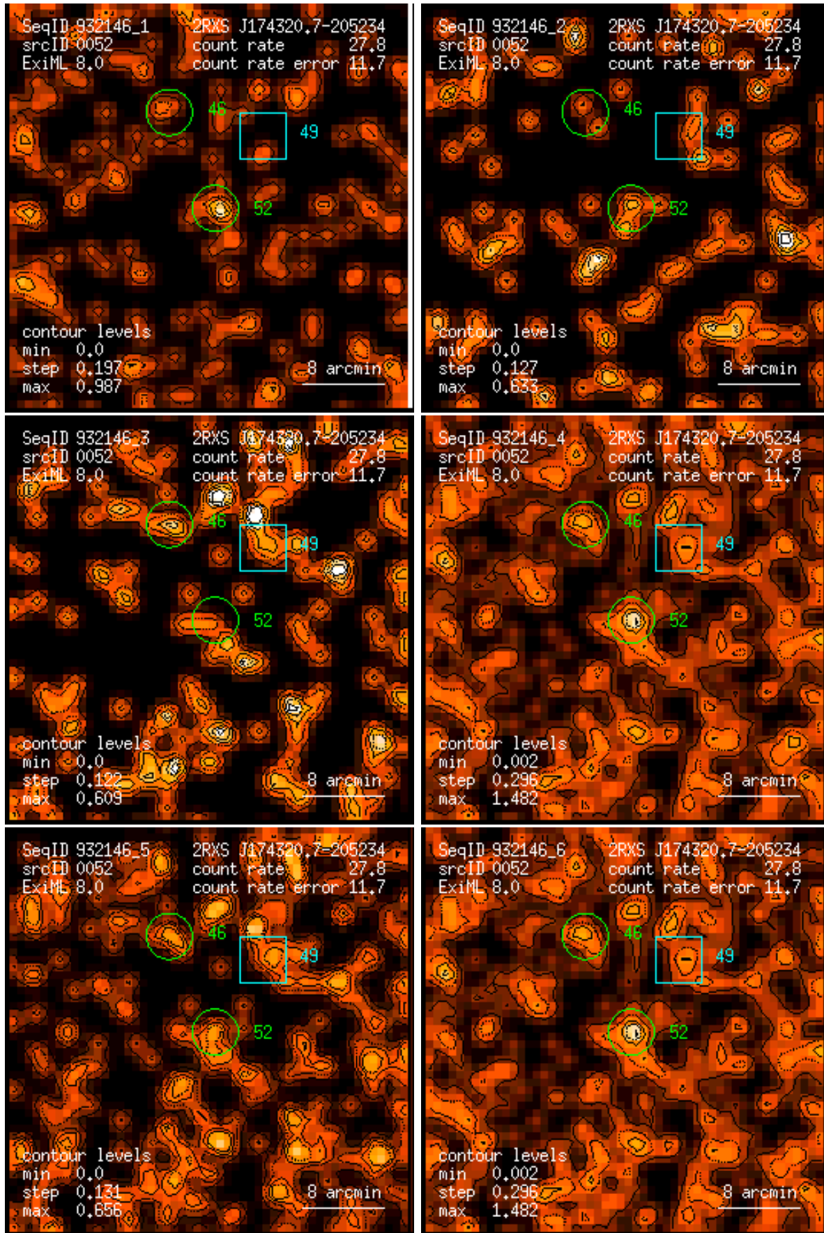
Figure 52: RASS 932146: detection 0052: band rate images, Gaussian filter: (1) PSPC channels 11 – 41, (2) 52 – 90, (3) 91 – 201, (4) 11 – 235, (5) 52 – 201, (6) 11 – 201. Broad band rates in counts/ks. Band rate contour levels in counts/ks/arcmin 2 .
