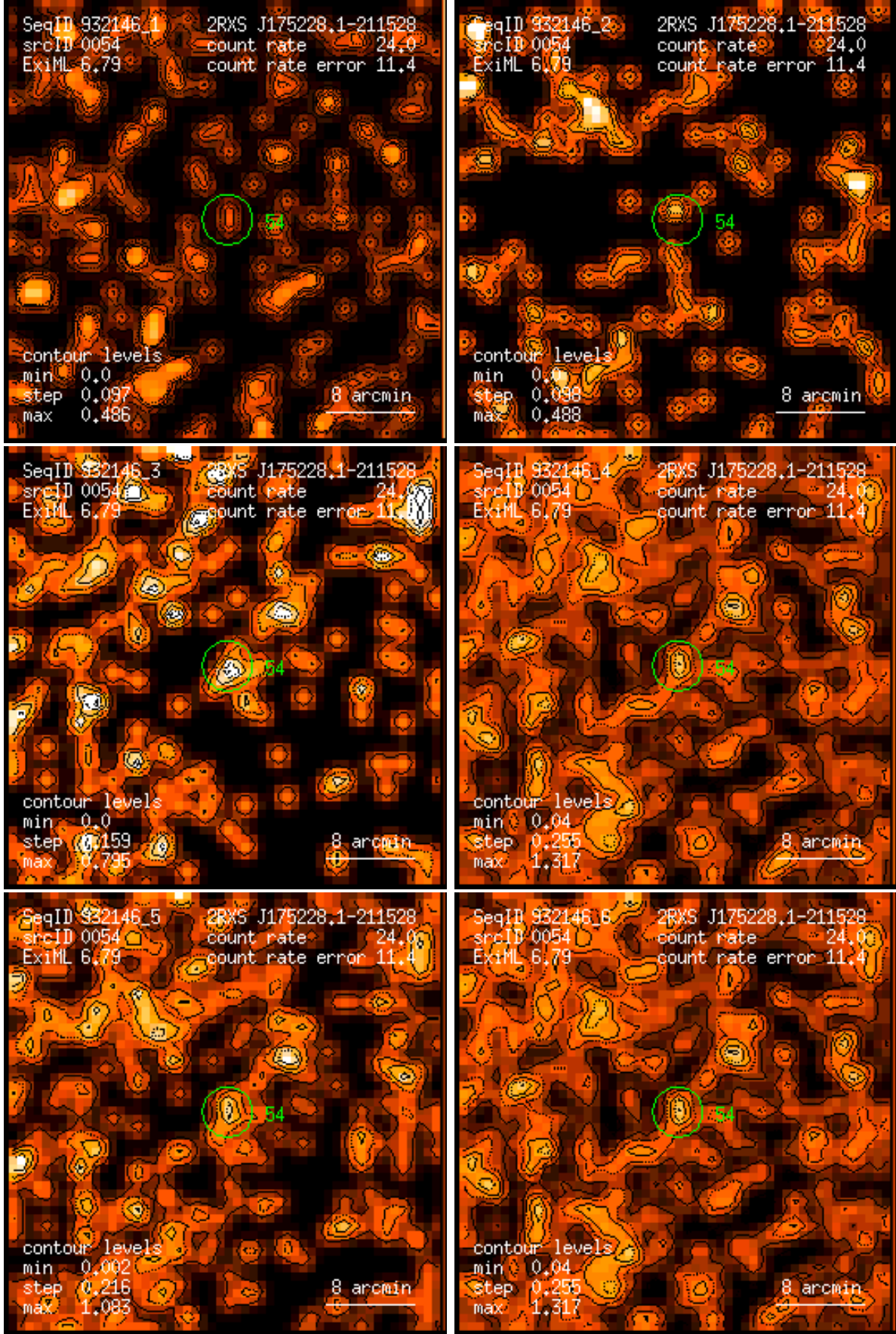
Figure 54: RASS 932146: detection 0054: band rate images, Gaussian filter: (1) PSPC channels 11 – 41, (2) 52 – 90, (3) 91 – 201, (4) 11 – 235, (5) 52 – 201, (6) 11 – 201. Broad band rates in counts/ks. Band rate contour levels in counts/ks/arcmin 2 .
