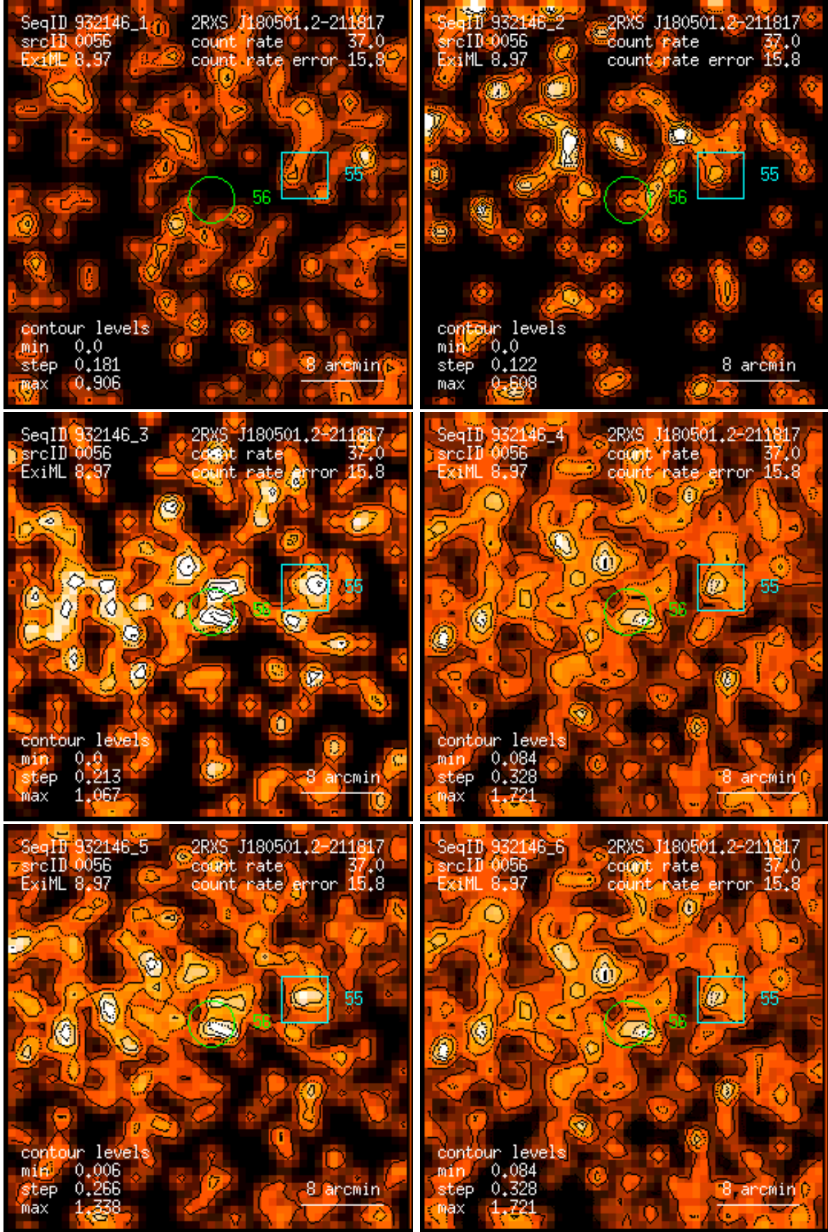
Figure 56: RASS 932146: detection 0056: band rate images, Gaussian filter: (1) PSPC channels 11 – 41, (2) 52 – 90, (3) 91 – 201, (4) 11 – 235, (5) 52 – 201, (6) 11 – 201. Broad band rates in counts/ks. Band rate contour levels in counts/ks/arcmin 2 .
