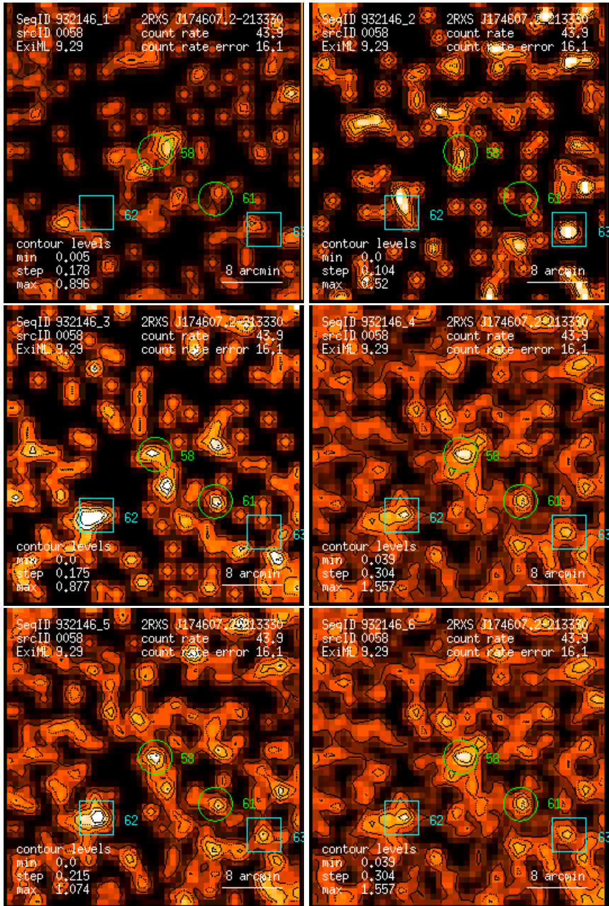
Figure 58: RASS 932146: detection 0058: band rate images, Gaussian filter: (1) PSPC channels 11 – 41, (2) 52 – 90, (3) 91 – 201, (4) 11 – 235, (5) 52 – 201, (6) 11 – 201. Broad band rates in counts/ks. Band rate contour levels in counts/ks/arcmin 2 .
