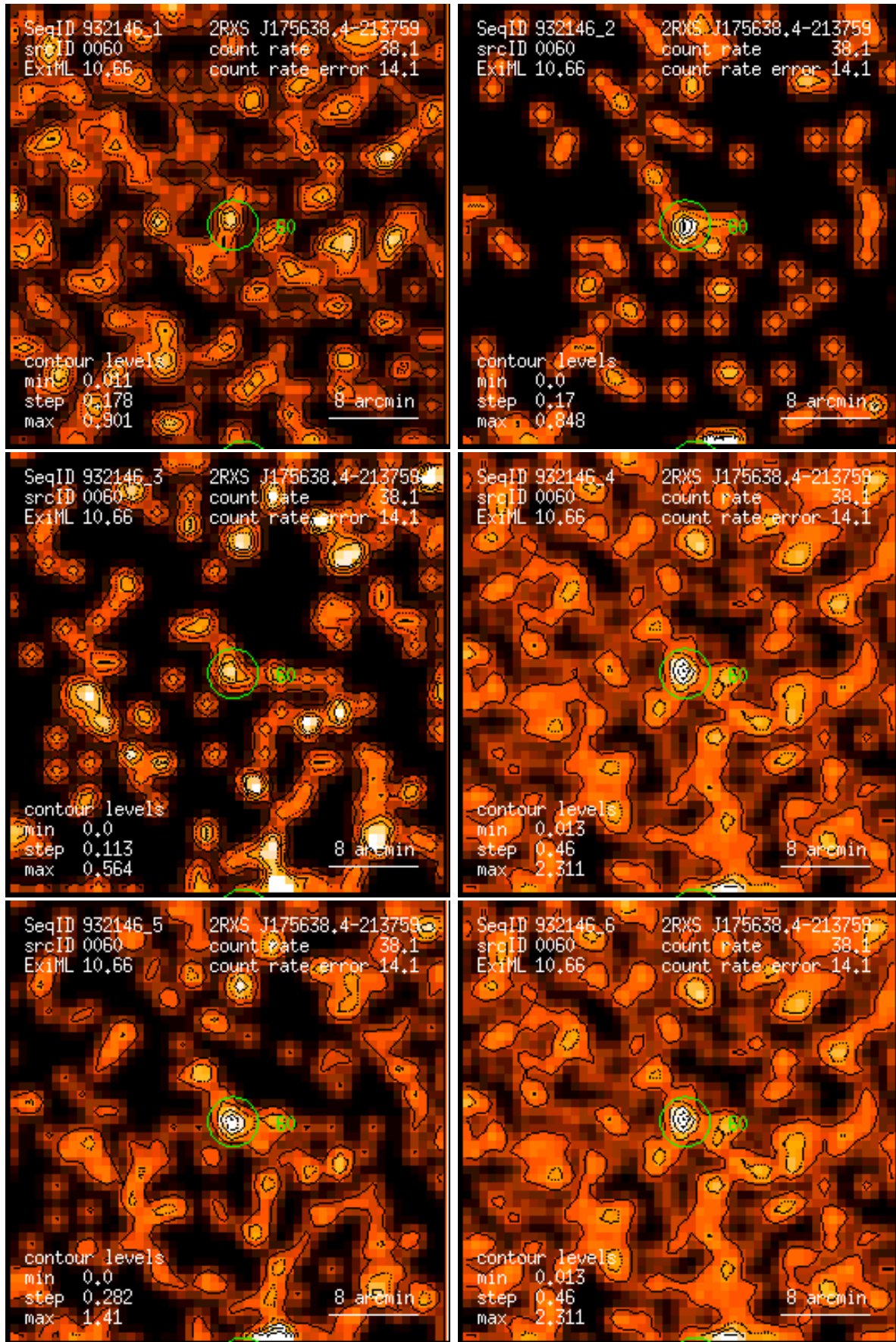
Figure 60: RASS 932146: detection 0060: band rate images, Gaussian filter: (1) PSPC channels 11 – 41, (2) 52 – 90, (3) 91 – 201, (4) 11 – 235, (5) 52 – 201, (6) 11 – 201. Broad band rates in counts/ks. Band rate contour levels in counts/ks/arcmin 2 .
