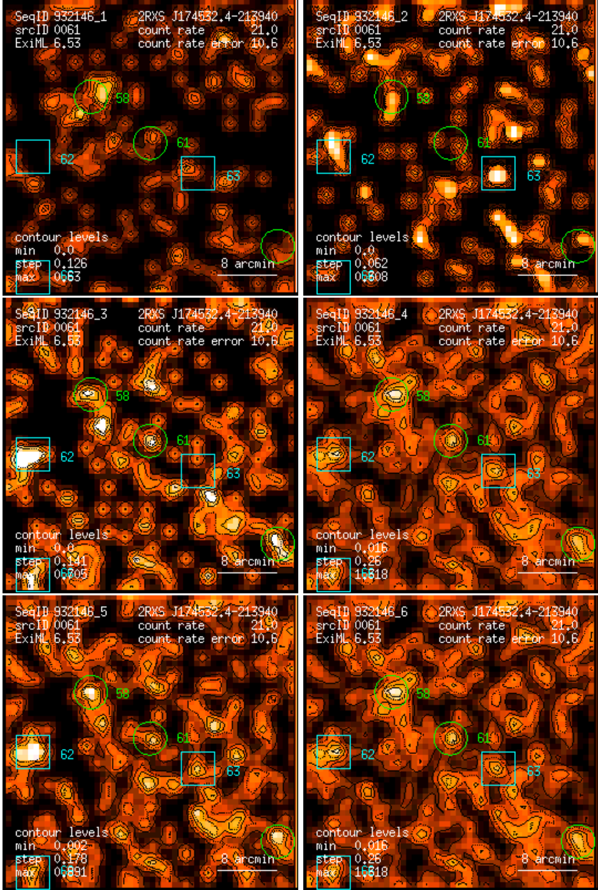
Figure 61: RASS 932146: detection 0061: band rate images, Gaussian filter: (1) PSPC channels 11 – 41, (2) 52 – 90, (3) 91 – 201, (4) 11 – 235, (5) 52 – 201, (6) 11 – 201. Broad band rates in counts/ks. Band rate contour levels in counts/ks/arcmin 2 .
