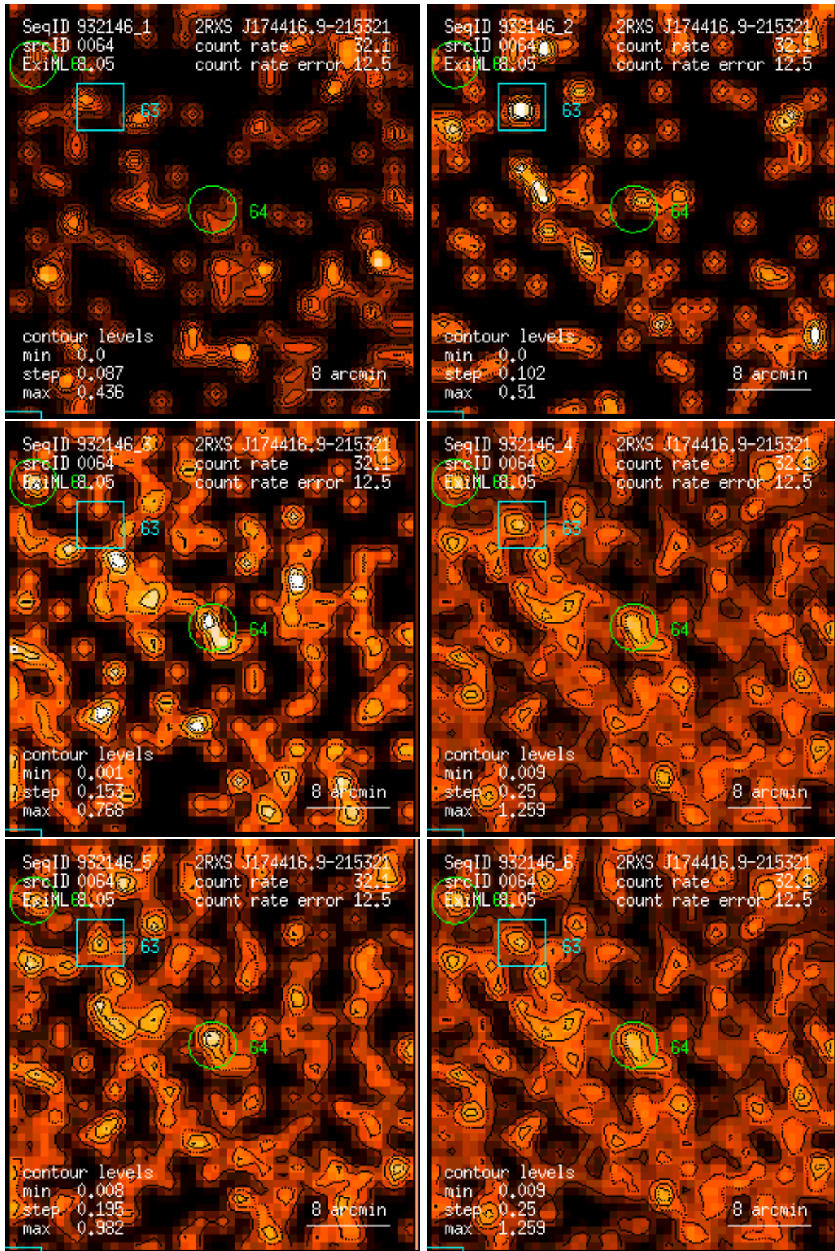
Figure 64: RASS 932146: detection 0064: band rate images, Gaussian filter: (1) PSPC channels 11 – 41, (2) 52 – 90, (3) 91 – 201, (4) 11 – 235, (5) 52 – 201, (6) 11 – 201. Broad band rates in counts/ks. Band rate contour levels in counts/ks/arcmin 2 .
