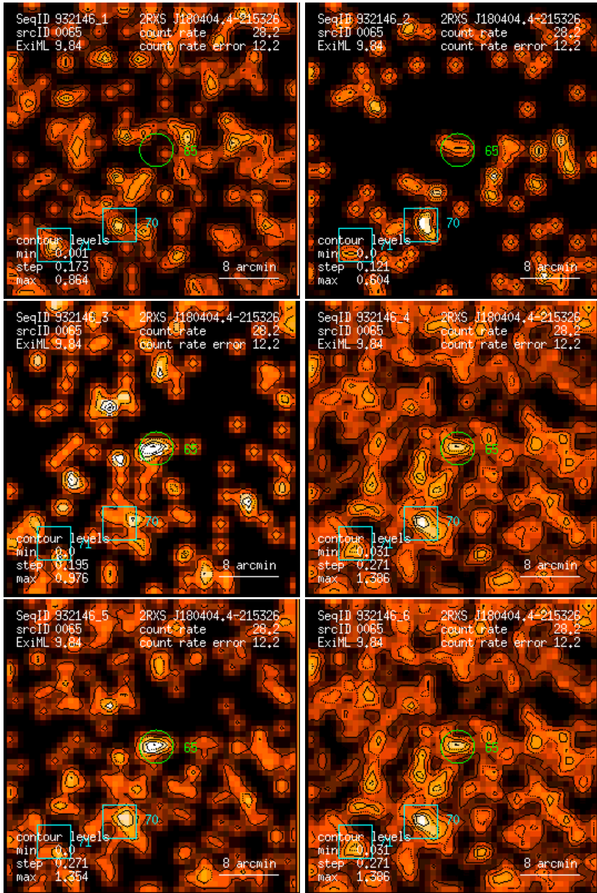
Figure 65: RASS 932146: detection 0065: band rate images, Gaussian filter: (1) PSPC channels 11 – 41, (2) 52 – 90, (3) 91 – 201, (4) 11 – 235, (5) 52 – 201, (6) 11 – 201. Broad band rates in counts/ks. Band rate contour levels in counts/ks/arcmin 2 .
