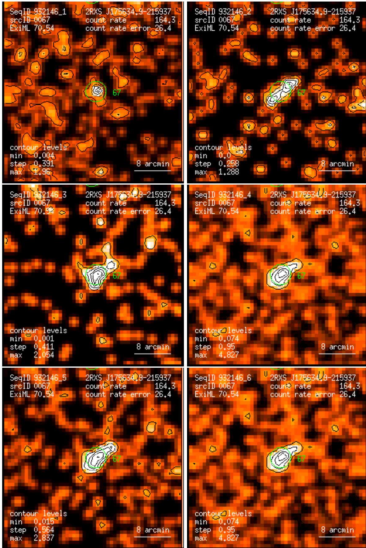
Figure 67: RASS 932146: detection 0067: band rate images, Gaussian filter: (1) PSPC channels 11 – 41, (2) 52 – 90, (3) 91 – 201, (4) 11 – 235, (5) 52 – 201, (6) 11 – 201. Broad band rates in counts/ks. Band rate contour levels in counts/ks/arcmin 2 .
