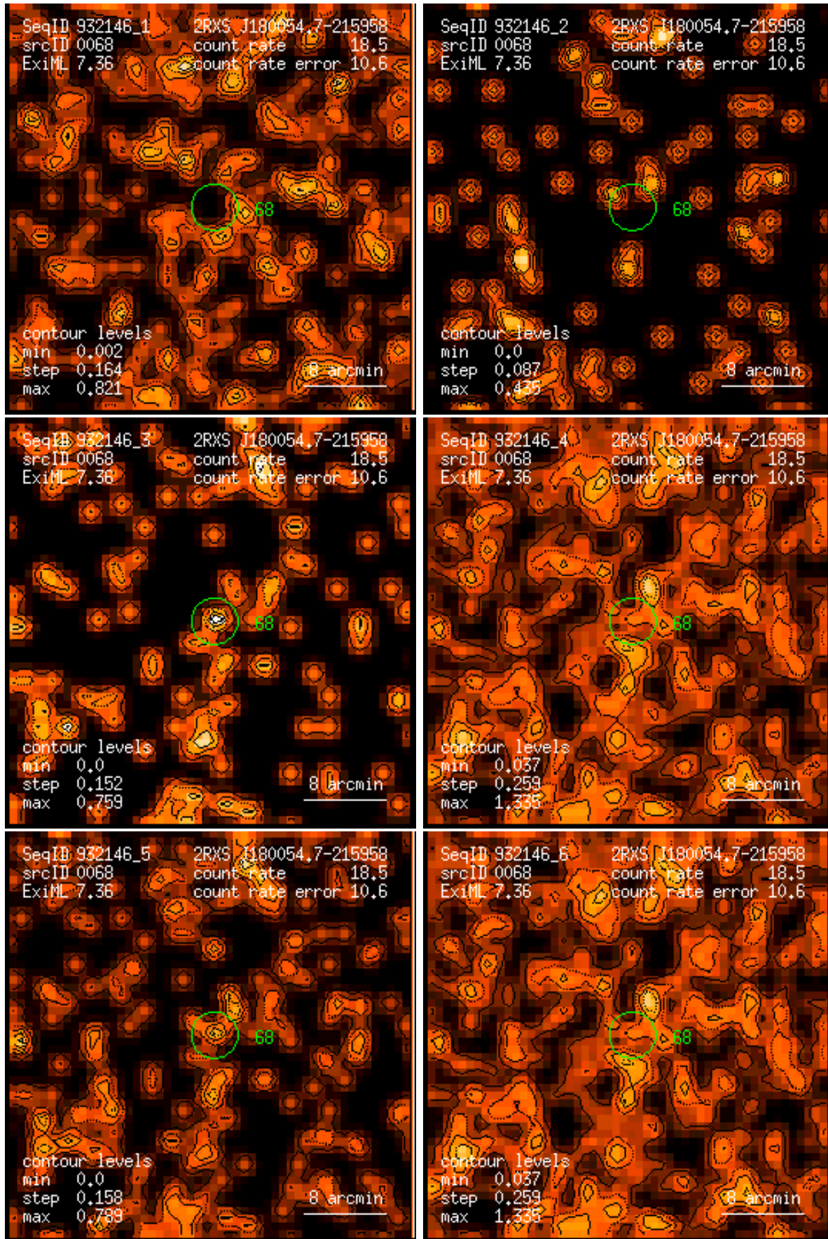
Figure 68: RASS 932146: detection 0068: band rate images, Gaussian filter: (1) PSPC channels 11 – 41, (2) 52 – 90, (3) 91 – 201, (4) 11 – 235, (5) 52 – 201, (6) 11 – 201. Broad band rates in counts/ks. Band rate contour levels in counts/ks/arcmin 2 .
