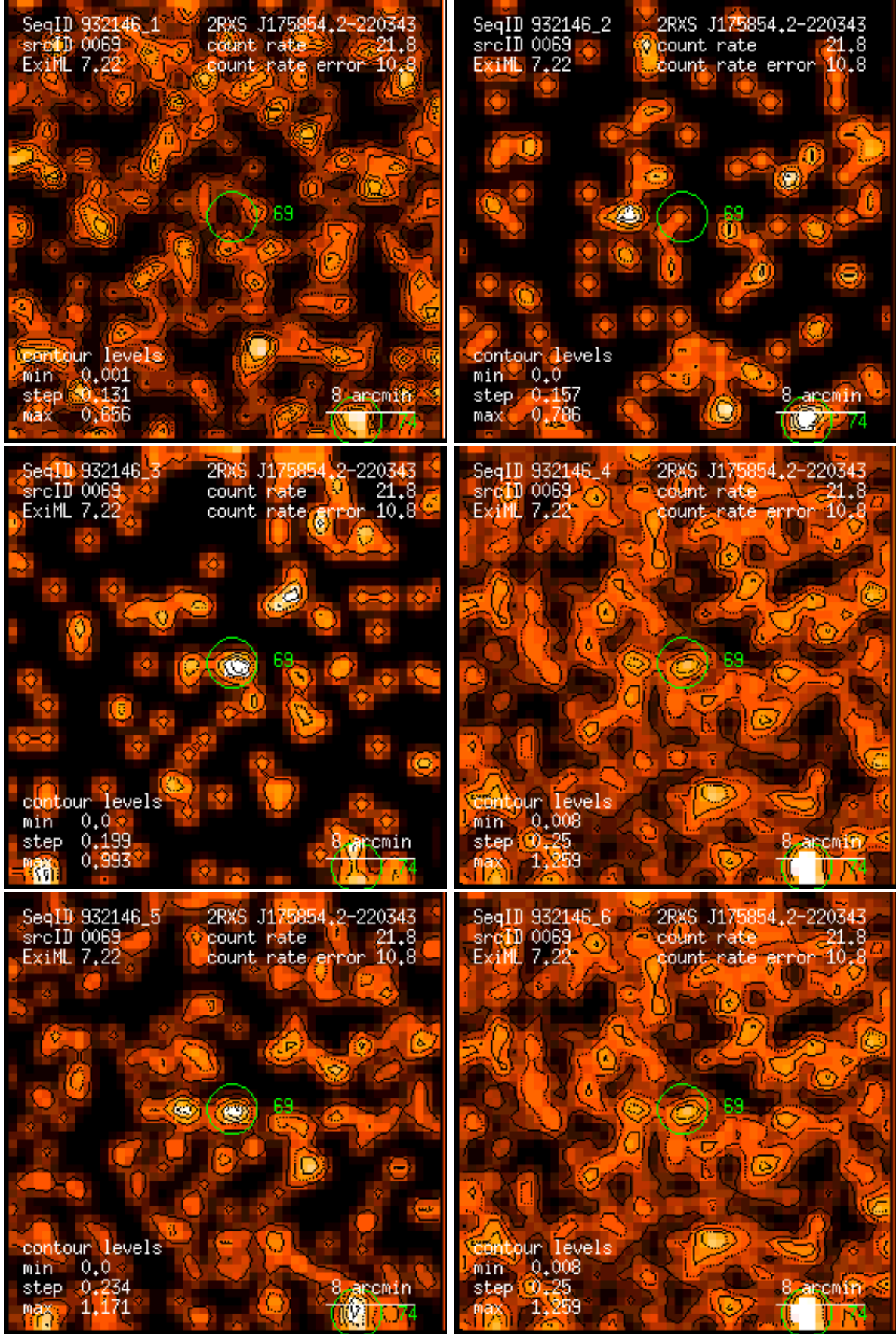
Figure 69: RASS 932146: detection 0069: band rate images, Gaussian filter: (1) PSPC channels 11 – 41, (2) 52 – 90, (3) 91 – 201, (4) 11 – 235, (5) 52 – 201, (6) 11 – 201. Broad band rates in counts/ks. Band rate contour levels in counts/ks/arcmin 2 .
