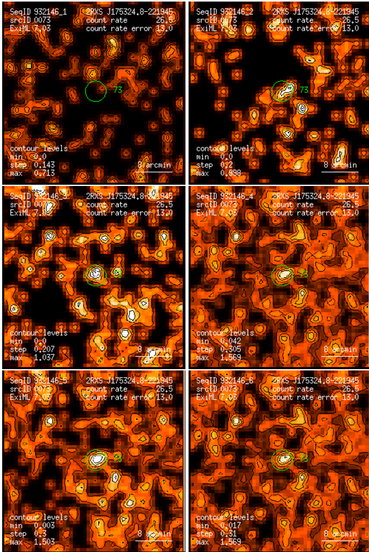
Figure 73: RASS 932146: detection 0073: band rate images, Gaussian filter: (1) PSPC channels 11 – 41, (2) 52 – 90, (3) 91 – 201, (4) 11 – 235, (5) 52 – 201, (6) 11 – 201. Broad band rates in counts/ks. Band rate contour levels in counts/ks/arcmin 2 .
