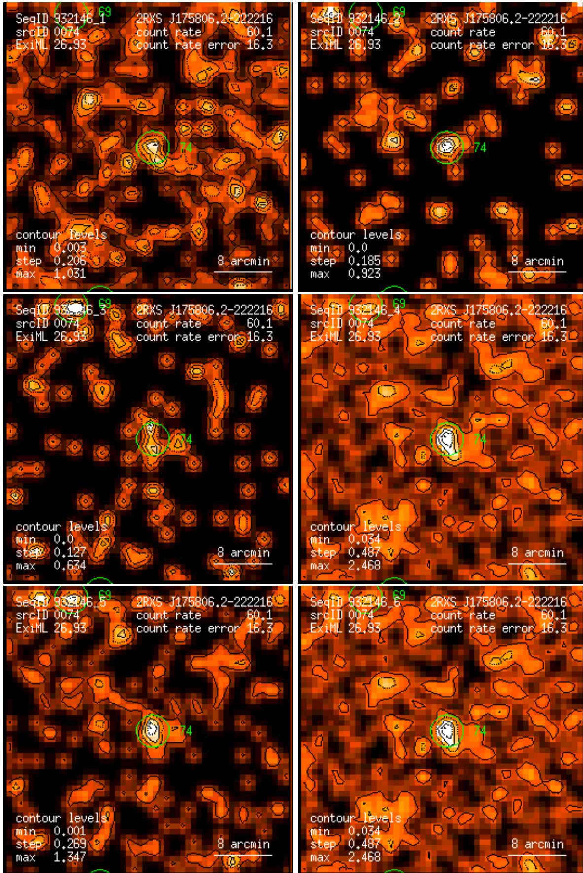
Figure 74: RASS 932146: detection 0074: band rate images, Gaussian filter: (1) PSPC channels 11 – 41, (2) 52 – 90, (3) 91 – 201, (4) 11 – 235, (5) 52 – 201, (6) 11 – 201. Broad band rates in counts/ks. Band rate contour levels in counts/ks/arcmin 2 .
