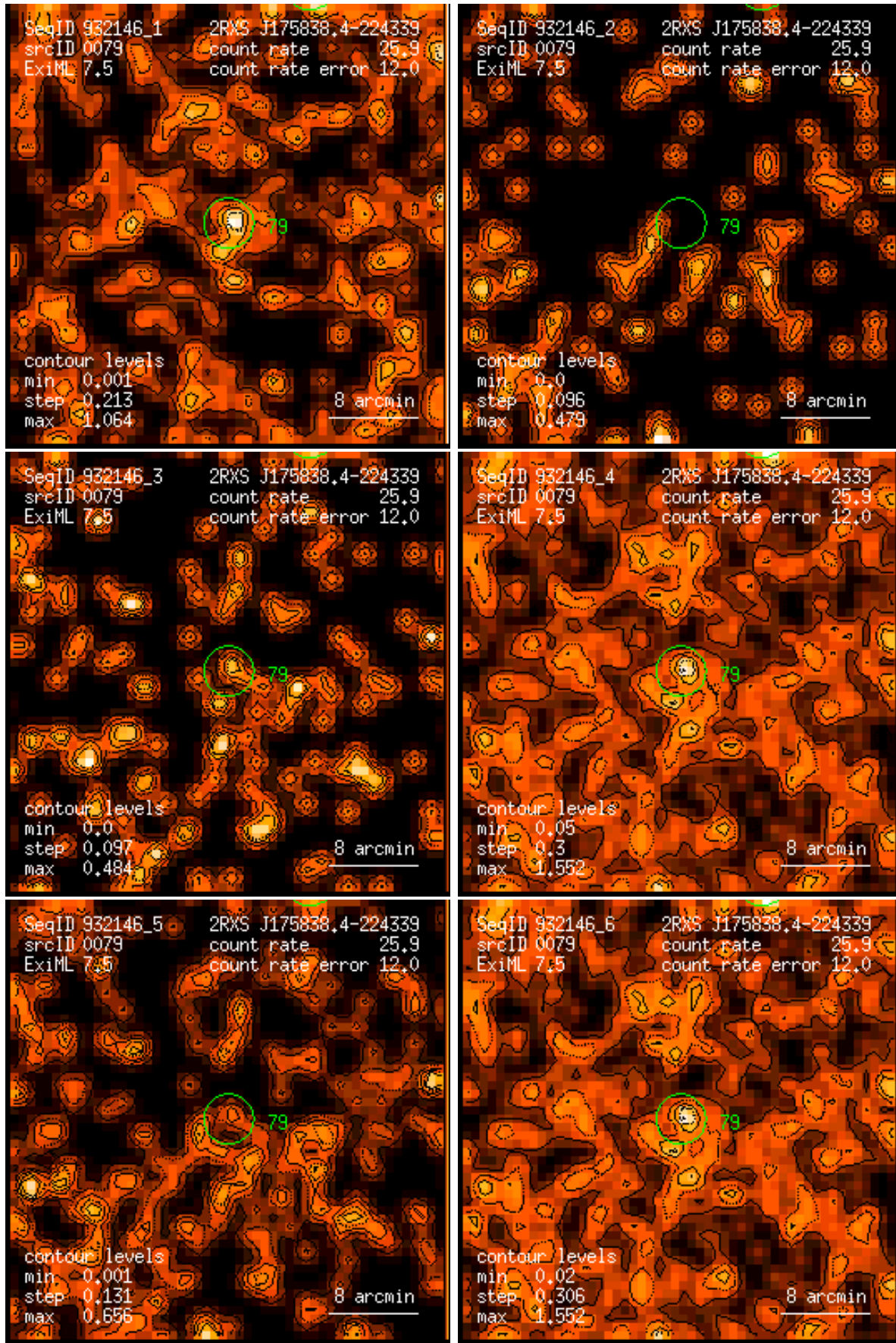
Figure 79: RASS 932146: detection 0079: band rate images, Gaussian filter: (1) PSPC channels 11 – 41, (2) 52 – 90, (3) 91 – 201, (4) 11 – 235, (5) 52 – 201, (6) 11 – 201. Broad band rates in counts/ks. Band rate contour levels in counts/ks/arcmin 2 .
