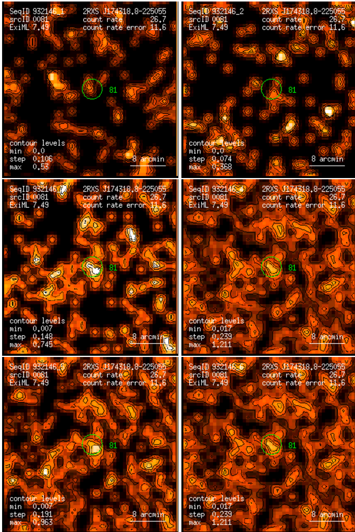
Figure 81: RASS 932146: detection 0081: band rate images, Gaussian filter: (1) PSPC channels 11 – 41, (2) 52 – 90, (3) 91 – 201, (4) 11 – 235, (5) 52 – 201, (6) 11 – 201. Broad band rates in counts/ks. Band rate contour levels in counts/ks/arcmin 2 .
