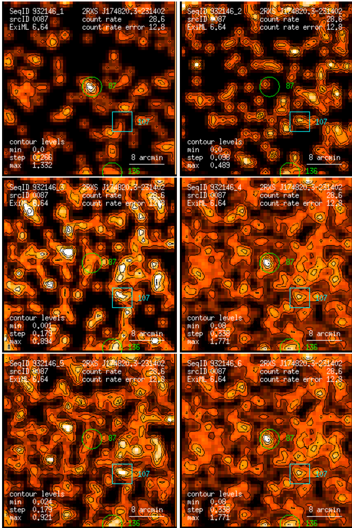
Figure 87: RASS 932146: detection 0087: band rate images, Gaussian filter: (1) PSPC channels 11 – 41, (2) 52 – 90, (3) 91 – 201, (4) 11 – 235, (5) 52 – 201, (6) 11 – 201. Broad band rates in counts/ks. Band rate contour levels in counts/ks/arcmin 2 .
