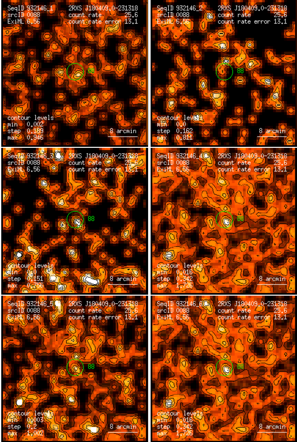
Figure 88: RASS 932146: detection 0088: band rate images, Gaussian filter: (1) PSPC channels 11 – 41, (2) 52 – 90, (3) 91 – 201, (4) 11 – 235, (5) 52 – 201, (6) 11 – 201. Broad band rates in counts/ks. Band rate contour levels in counts/ks/arcmin 2 .
