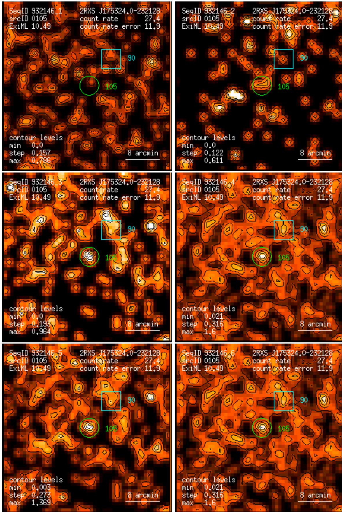
Figure 105: RASS 932146: detection 0105: band rate images, Gaussian filter: (1) PSPC channels 11 – 41, (2) 52 – 90, (3) 91 – 201, (4) 11 – 235, (5) 52 – 201, (6) 11 – 201. Broad band rates in counts/ks. Band rate contour levels in counts/ks/arcmin 2 .
